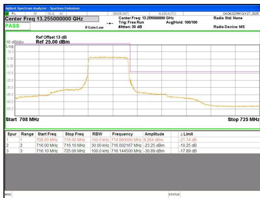
Band 12 3MHz/714.5/High QPSK 1@0
