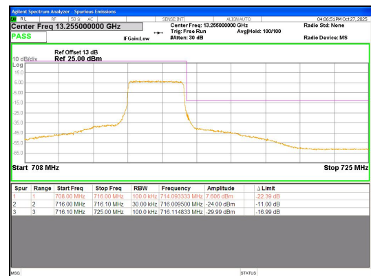
Band 12 3MHz/714.5/High 16QAM 1@0
