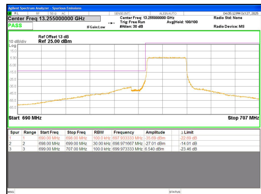
Band 12 3MHz/700.5/Low 16QAM 1@0
