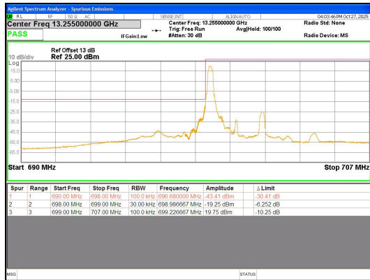
Band 12 3MHz/700.5/Low QPSK 1@0
