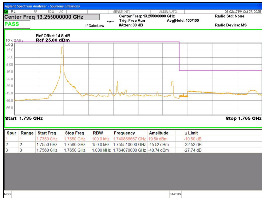
Band 4 15MHz/1747.5/High QPSK 1@0
