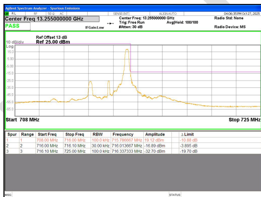
Band 12 3MHz/714.5/High QPSK 15@0
