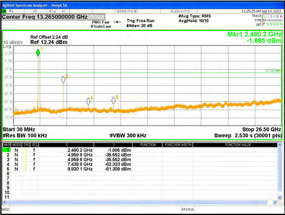
Tx. Spurious NVNT BLE 1M 2480MHz Ant3 Emission
