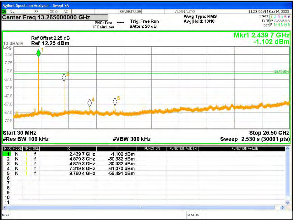
Tx. Spurious NVNT BLE 1M 2440MHz Ant3 Emission
