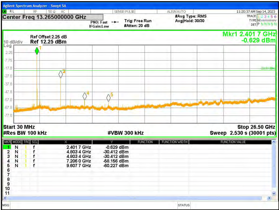
Tx. Spurious NVNT BLE 1M 2402MHz Ant3 Emission
