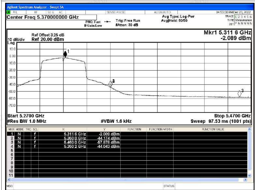
Restrict Band NVNT ac40 5310MHz Ant1 Average
