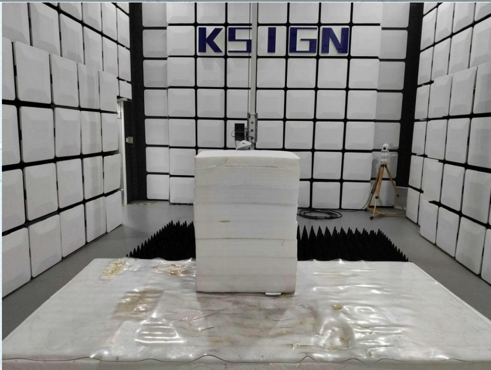
Emissions in restricted frequency bands (above 1GHz)
