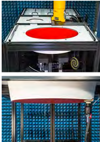
Figure 2.6 Flat Phantom
