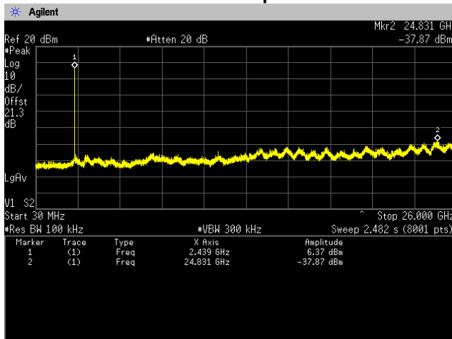
802.11b Ch 6 Spurious
