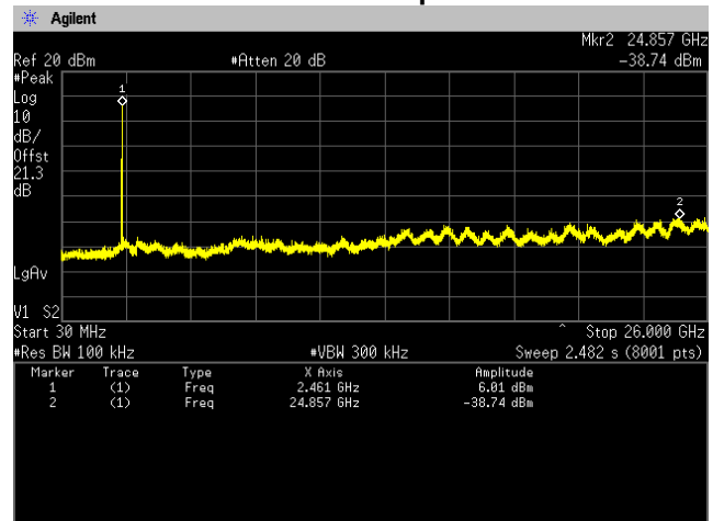
802.11b Ch 11 Spurious
