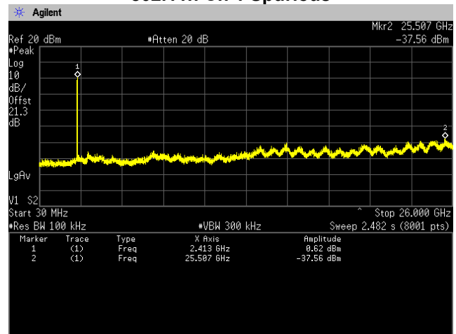
802.11n Ch 1 Spurious
