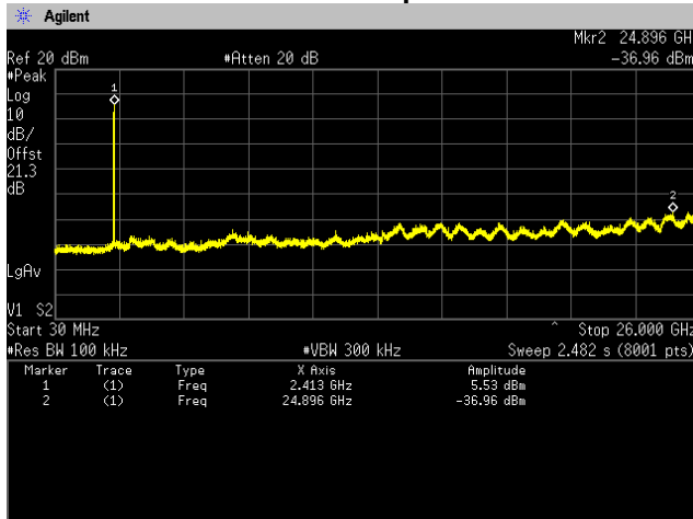
802.11b Ch 1 Spurious
