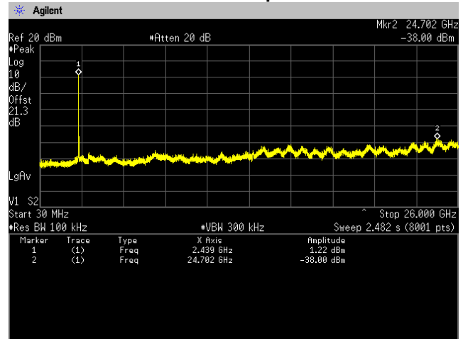
802.11n Ch 6 Spurious
