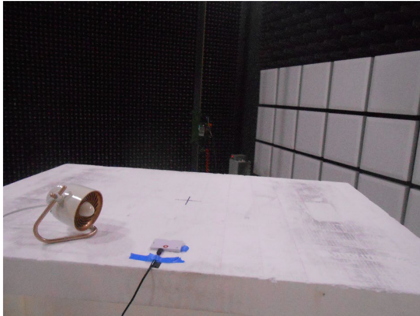
Radiated Emissions above 1 GHz (2)
