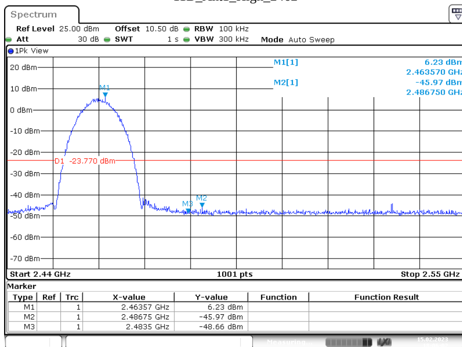
11B_Ant1_High_2462
