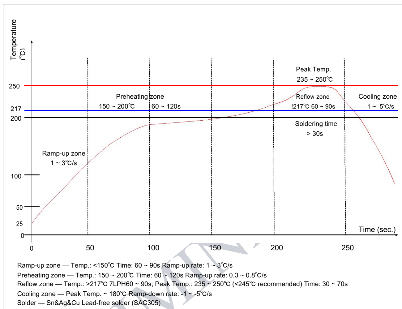
Figure 2: Reflow Profile
