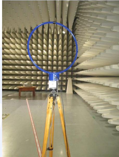
Radiated disturbance
