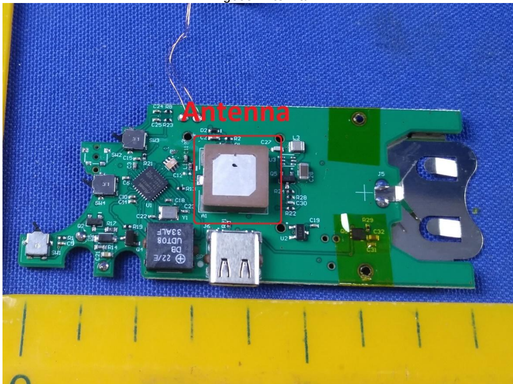
Zigbee Antenna
