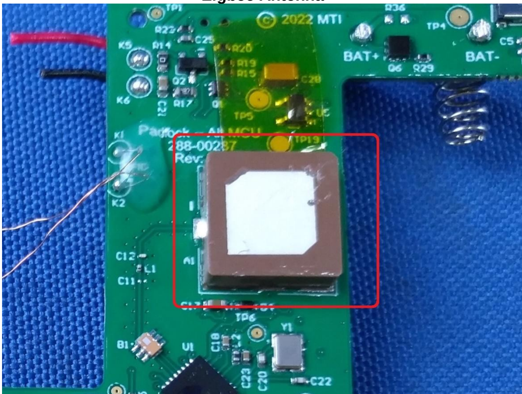
Zigbee Antenna
