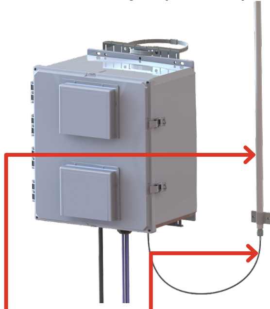
Antenna Assembly #2 (continued)
