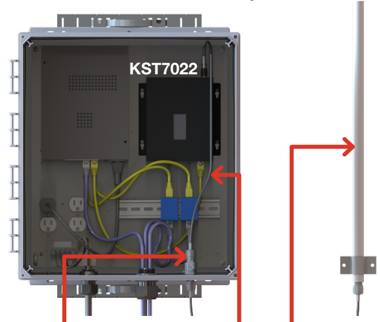
Antenna Assembly #3
