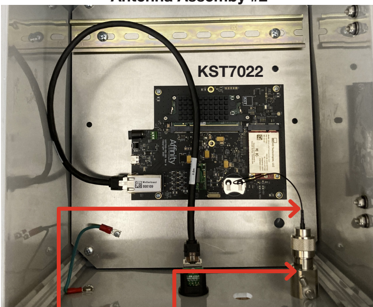
Antenna Assembly #2
