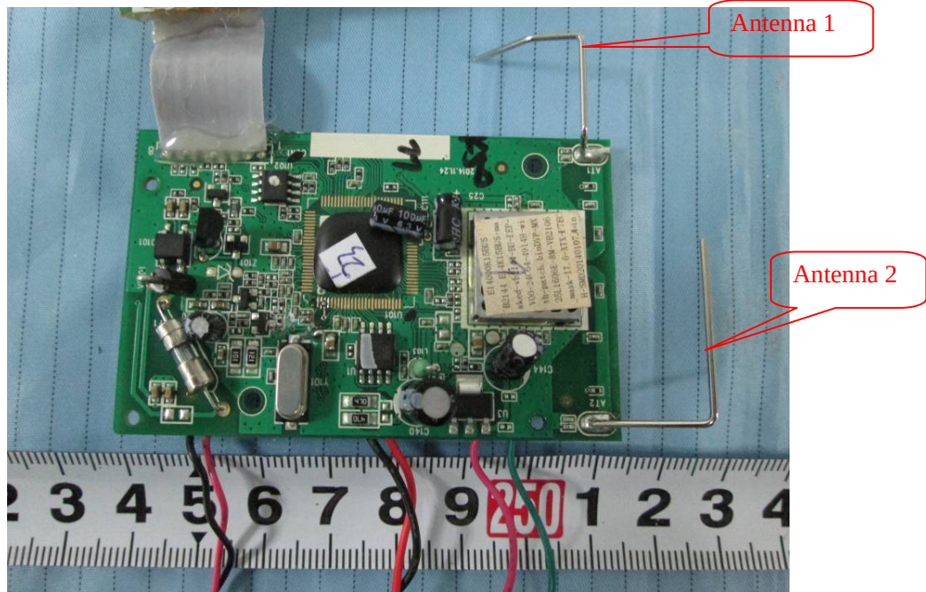
EUT –Main Board 2 Top View
