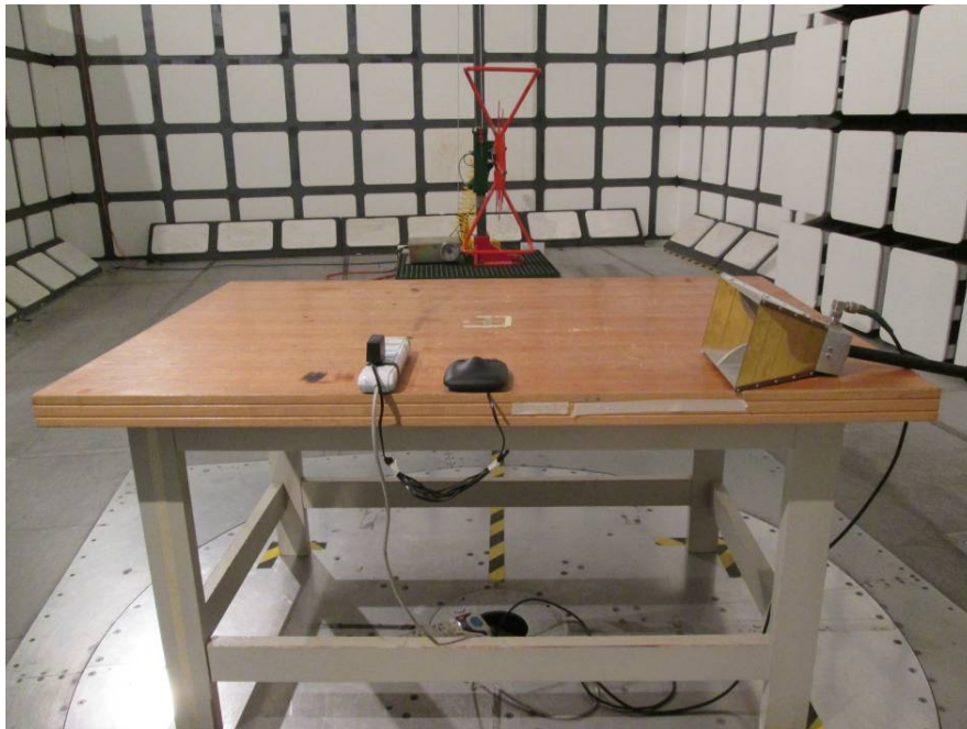
Radiated Emissions - Side View (Below 1 GHz)
