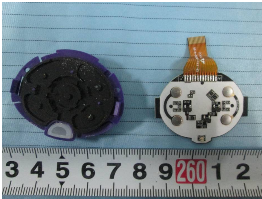
EUT – Control Panel Cover off View
