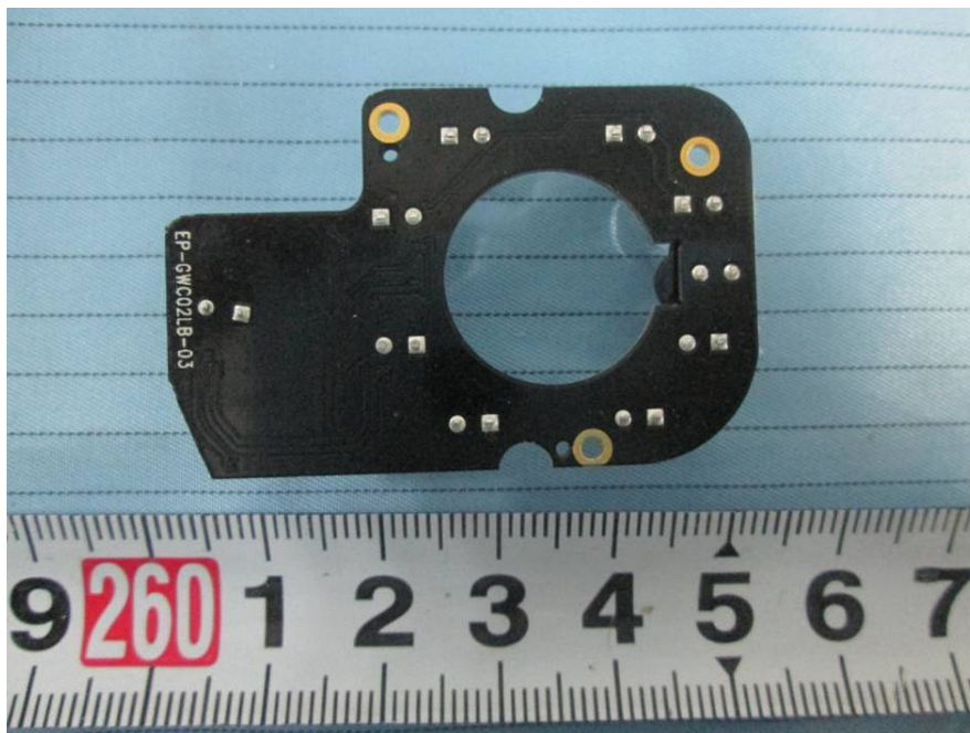
EUT –Camera Plate Bottom View
