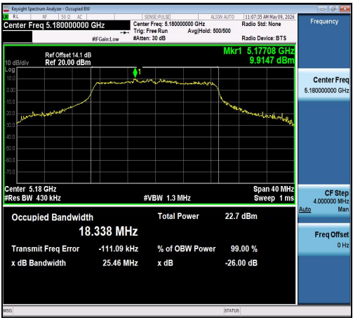
11AC20MIMO-Ant0-5180
