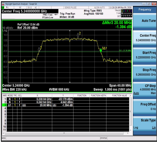
11AC20MIMO-Ant1-5240
