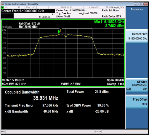
11AC40MIMO-Ant1-5190
