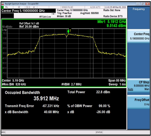
11AC40MIMO-Ant0-5190
