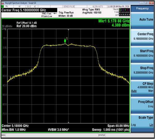
11AC20MIMO-Ant0-5180-PASS
