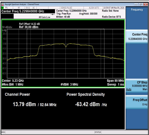
11N40MIMO-Ant0-5230-PASS
