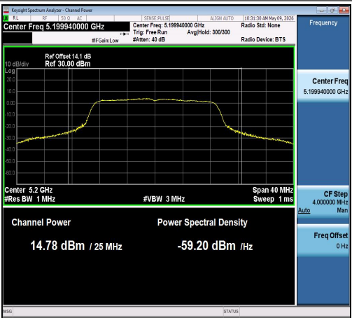
11N20MIMO-Ant0-5200-PASS
