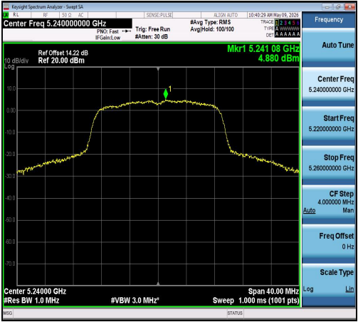
11N20MIMO-Ant0-5240-PASS
