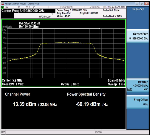
11AC20MIMO-Ant1-5200-PASS
