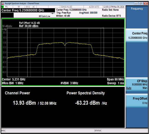
11AC40MIMO-Ant0-5230-PASS
