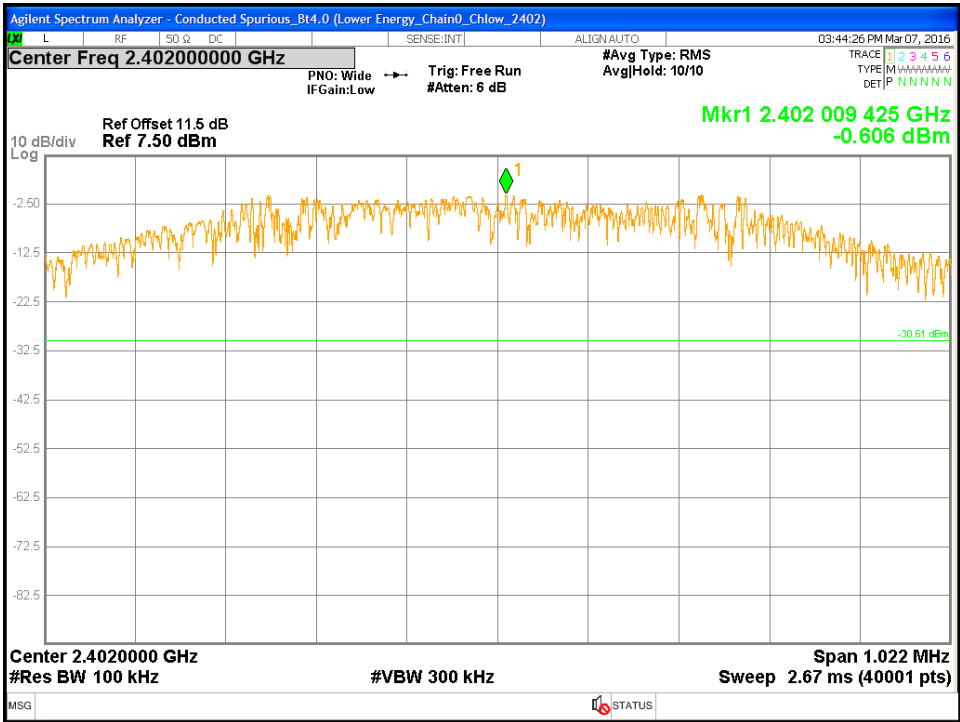
Chain0 : Conducted Spurious @ Lower Energy mode Ch low
