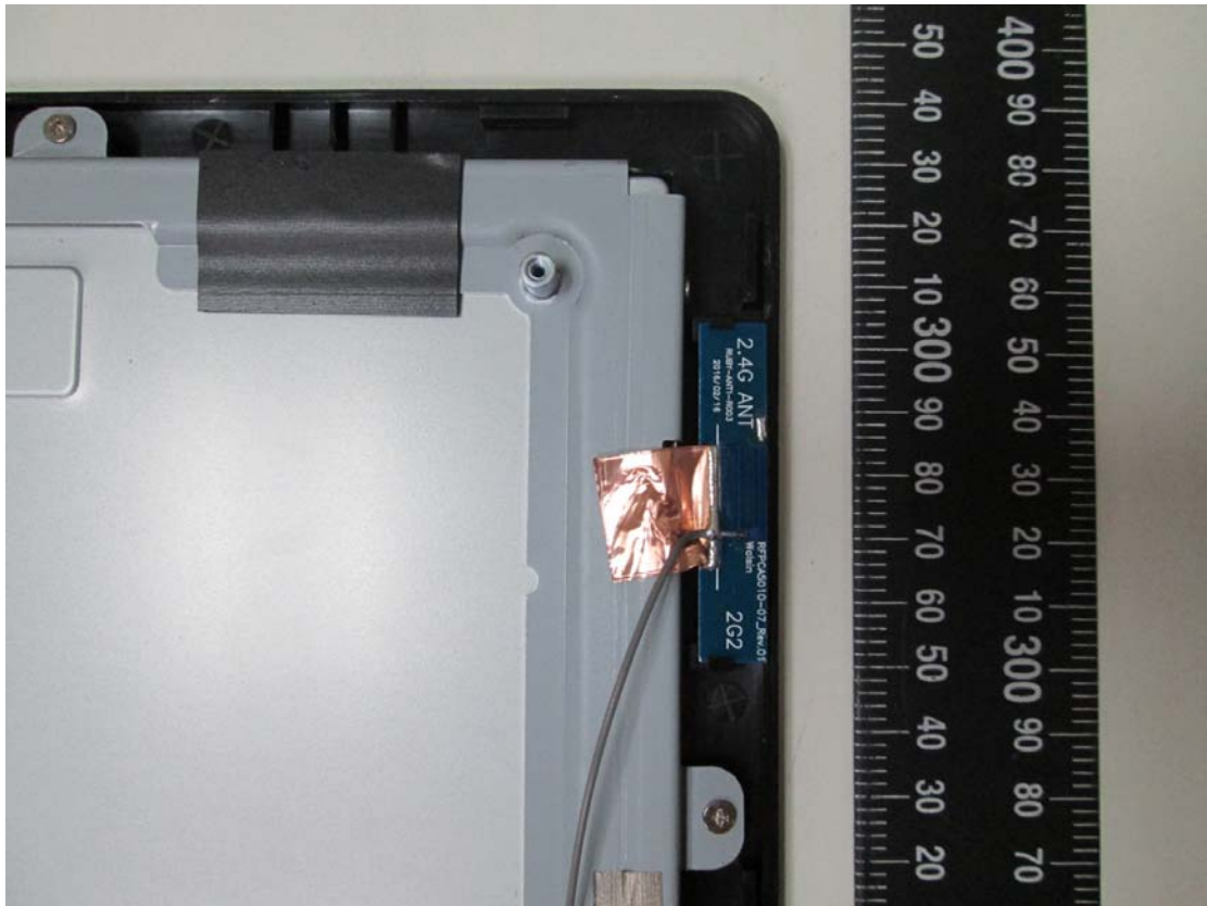
Ant+ Antenna
