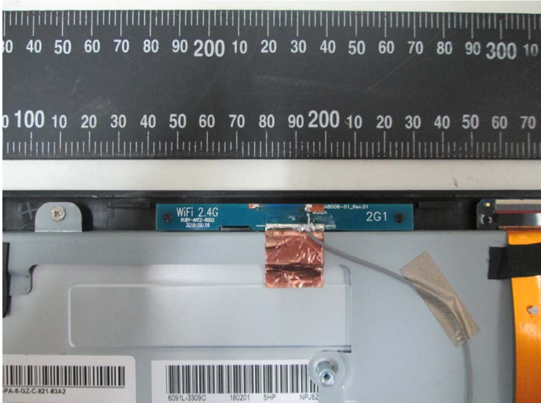
WiFi Antenna
