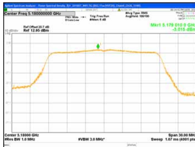
Chain0 : Power Spectral Density @ 802.11ac(VHT20) Mode Ch36
