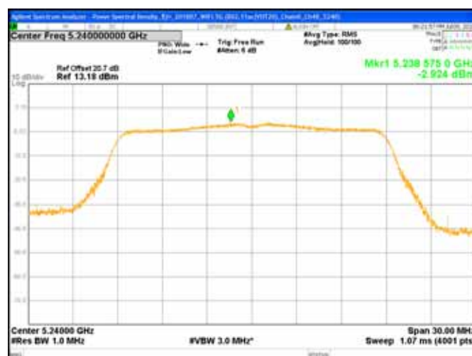
Chain0 : Power Spectral Density @ 802.11ac(VHT20) Mode Ch48
