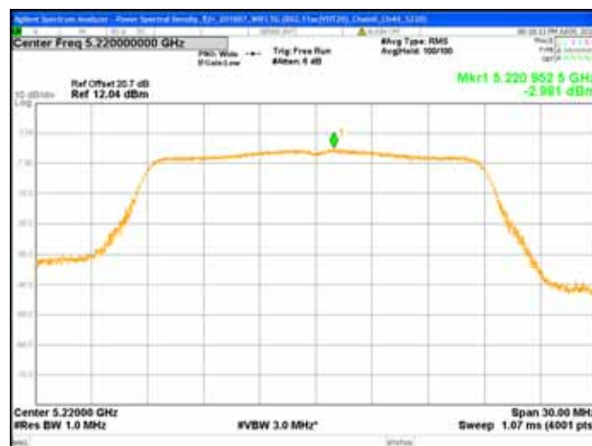
Chain0 : Power Spectral Density @ 802.11ac(VHT20) Mode Ch44
