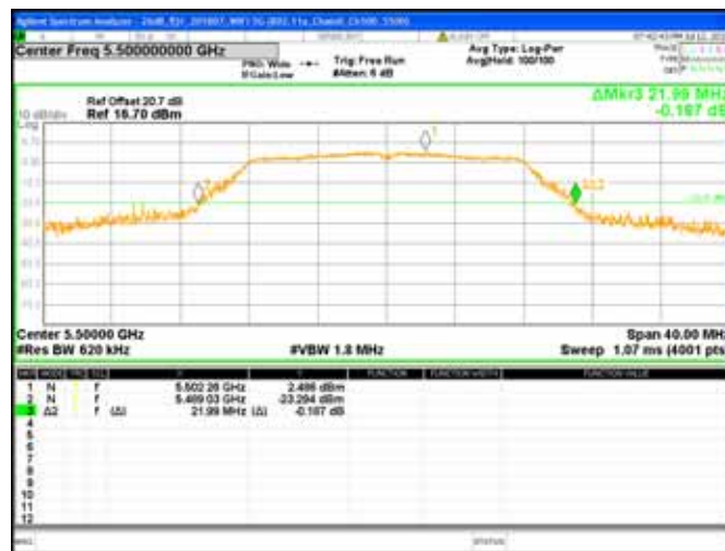
Chain0 : 26dB Bandwidth @ 802.11a Mode Ch100
