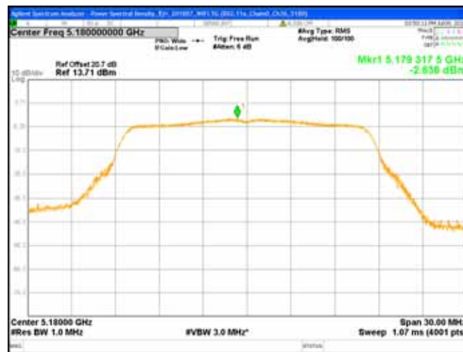
Chain0 : Power Spectral Density @ 802.11a Mode Ch36
