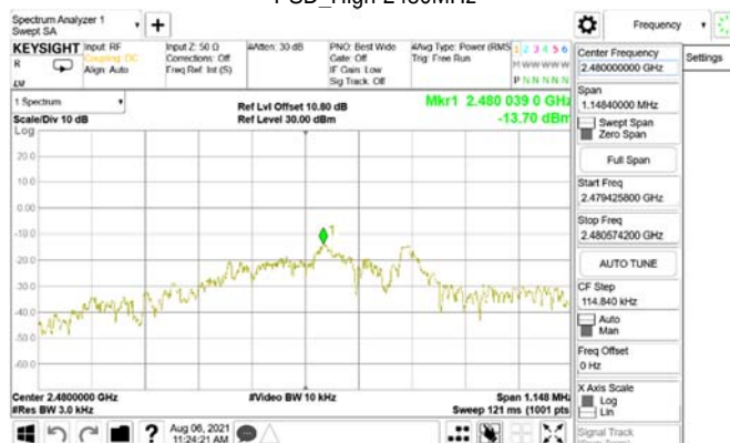
PSD_High-2480MHz
