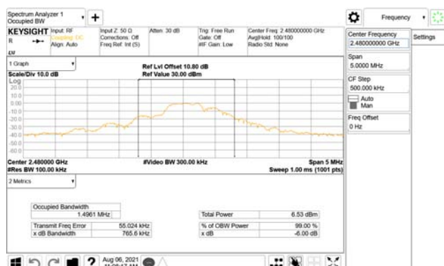
OBW_High-2480MHz
