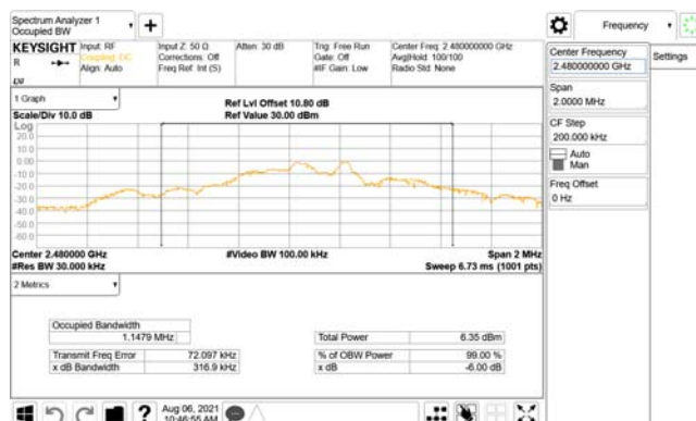
IC OBW_High-2480MHz
