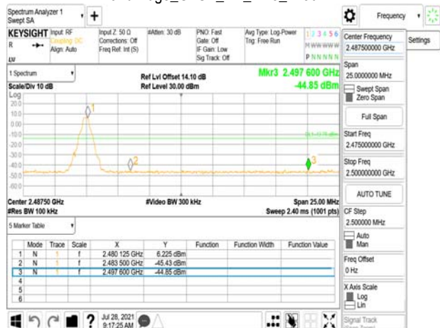
Band Edge_GFSK_1M_DH5_2480MHz
