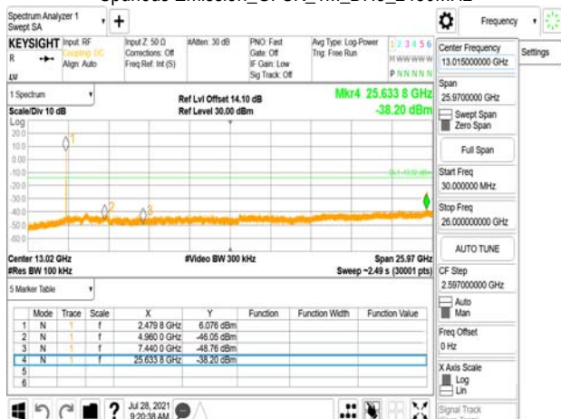
Spurious Emission_GFSK_1M_DH5_2480MHz
