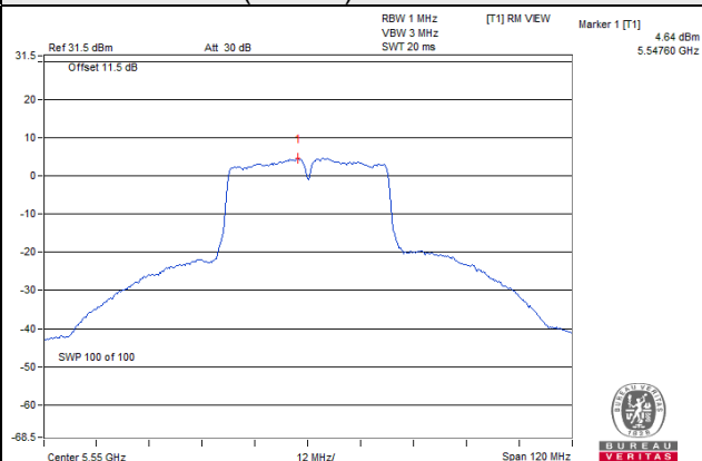
802.11ac (VHT40) / Chain 1 / CH 110
