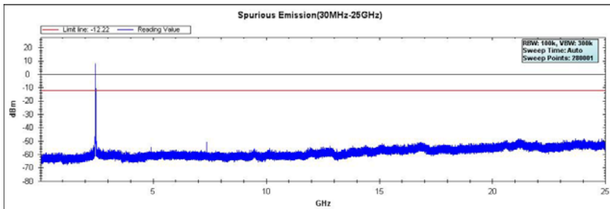
Channel 11 (2462MHz)
