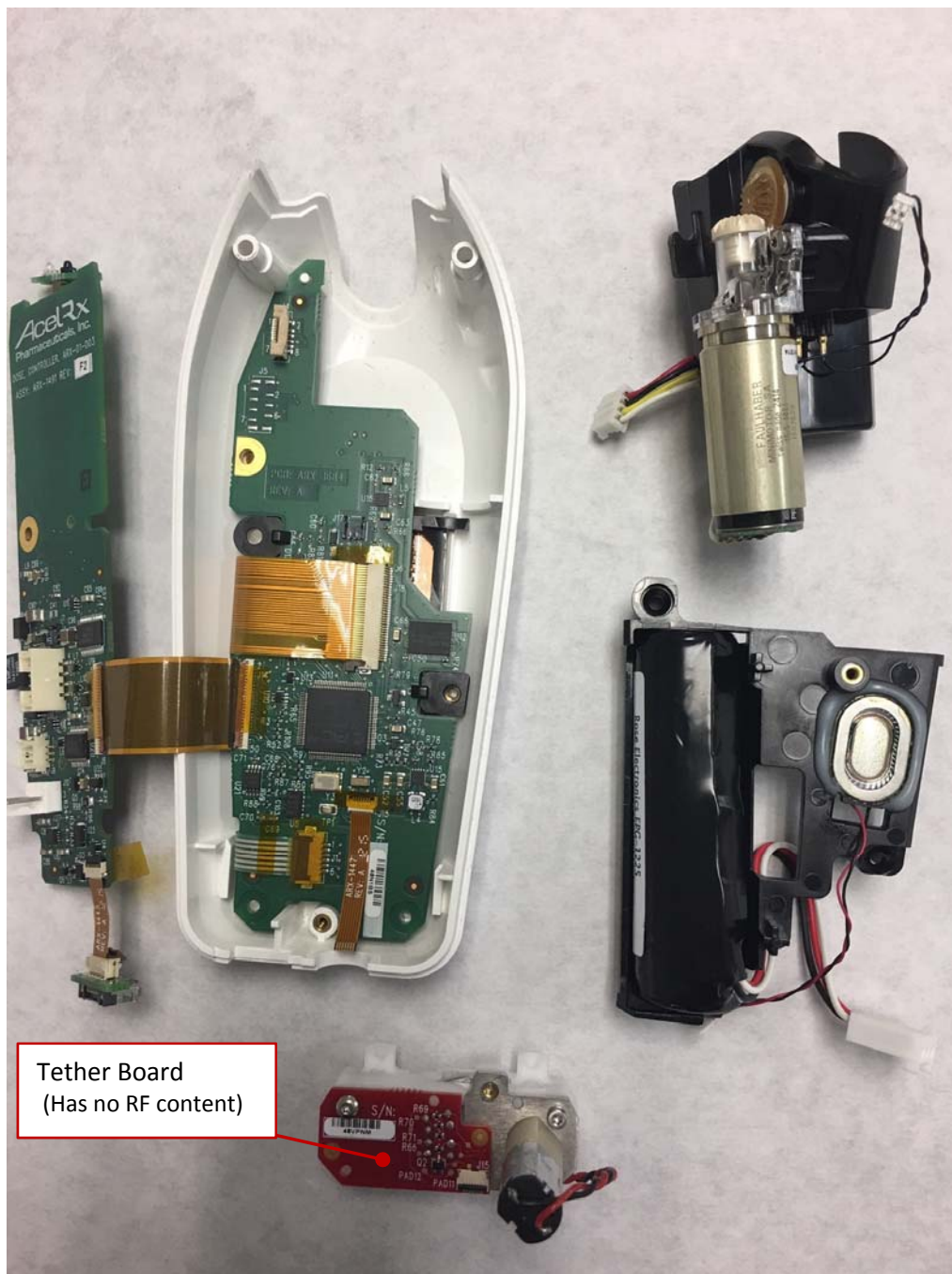
Figure 5: Disassembled Zalviso Controller
