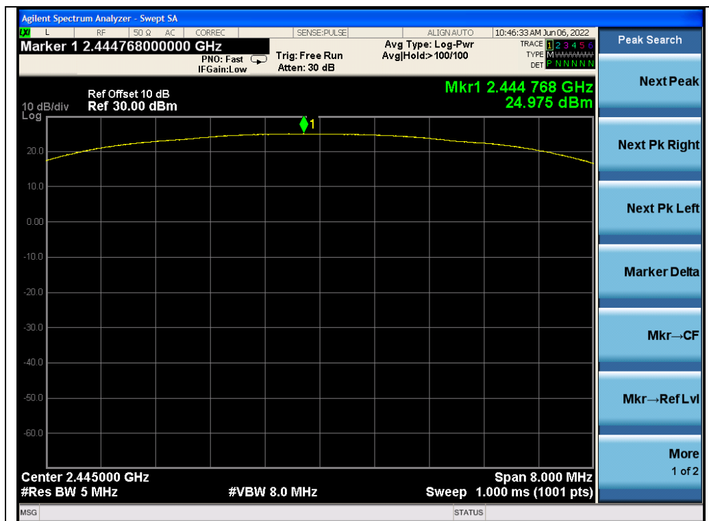
Test_Graph_GFSK_ANT1_2445_Peak Power
