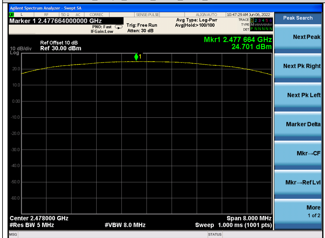
Test_Graph_GFSK_ANT1_2478_Peak Power
