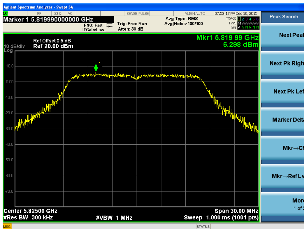
Test Plot For 802.11a-5825M-Chain 3
