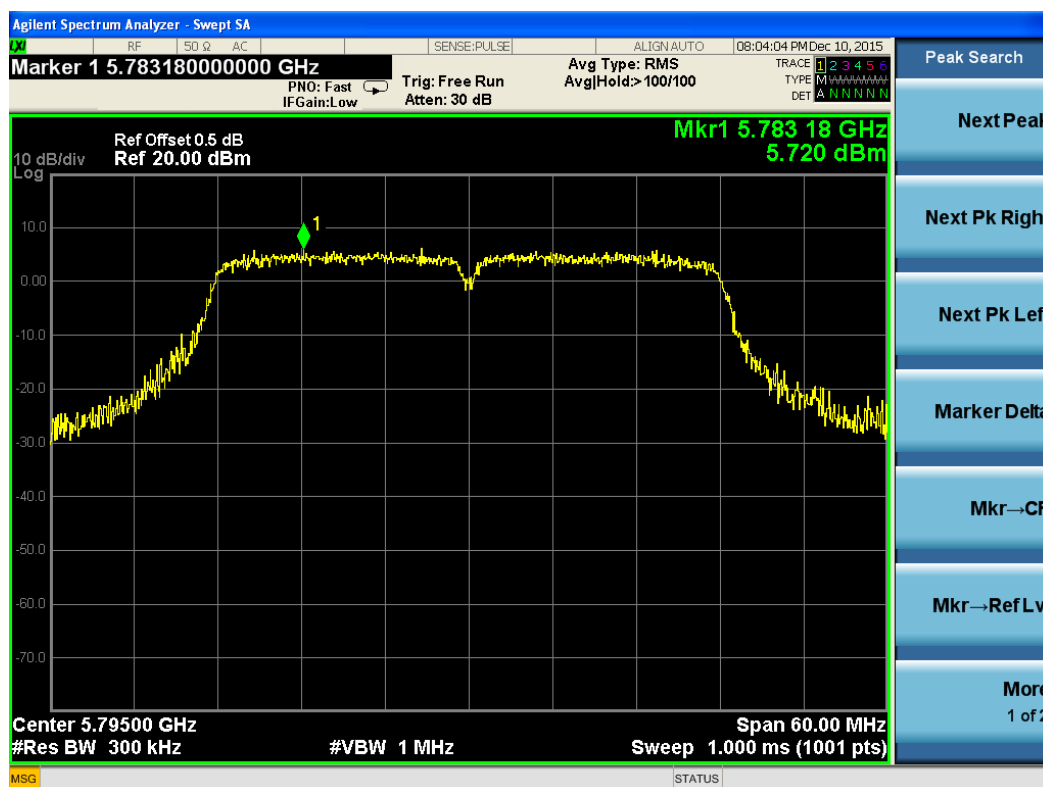
Test Plot For 802.11n(HT40)-5795M-Chain 1
