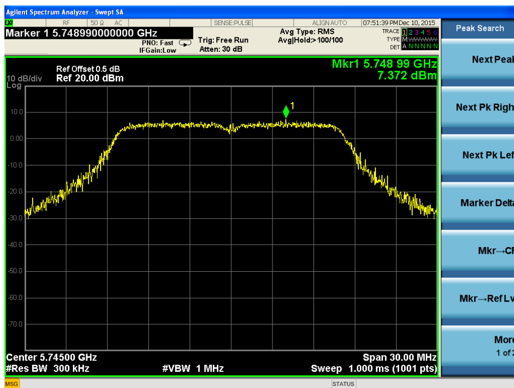
Test Plot For 802.11a-5745M-Chain 3
