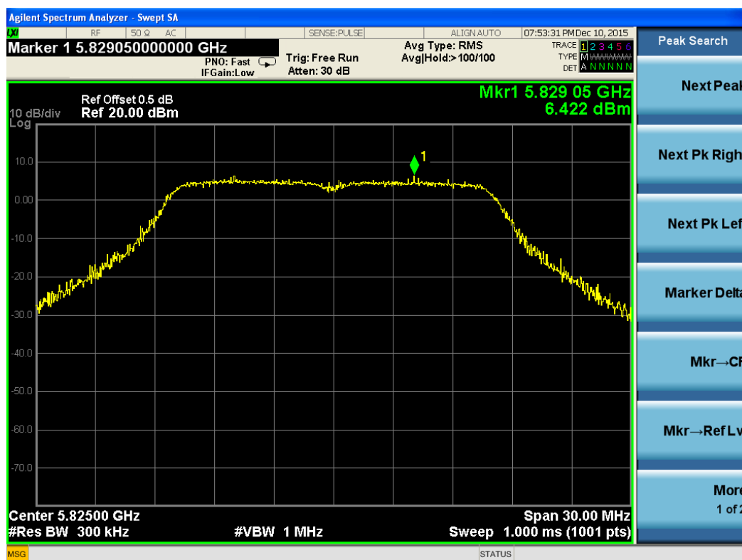
Test Plot For 802.11a-5825M-Chain 1
