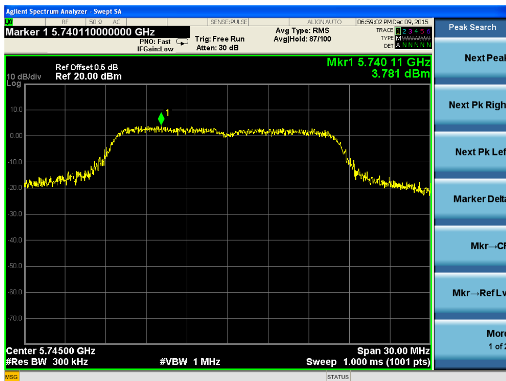
Test Plot For 802.11a-5745M-Chain 2
