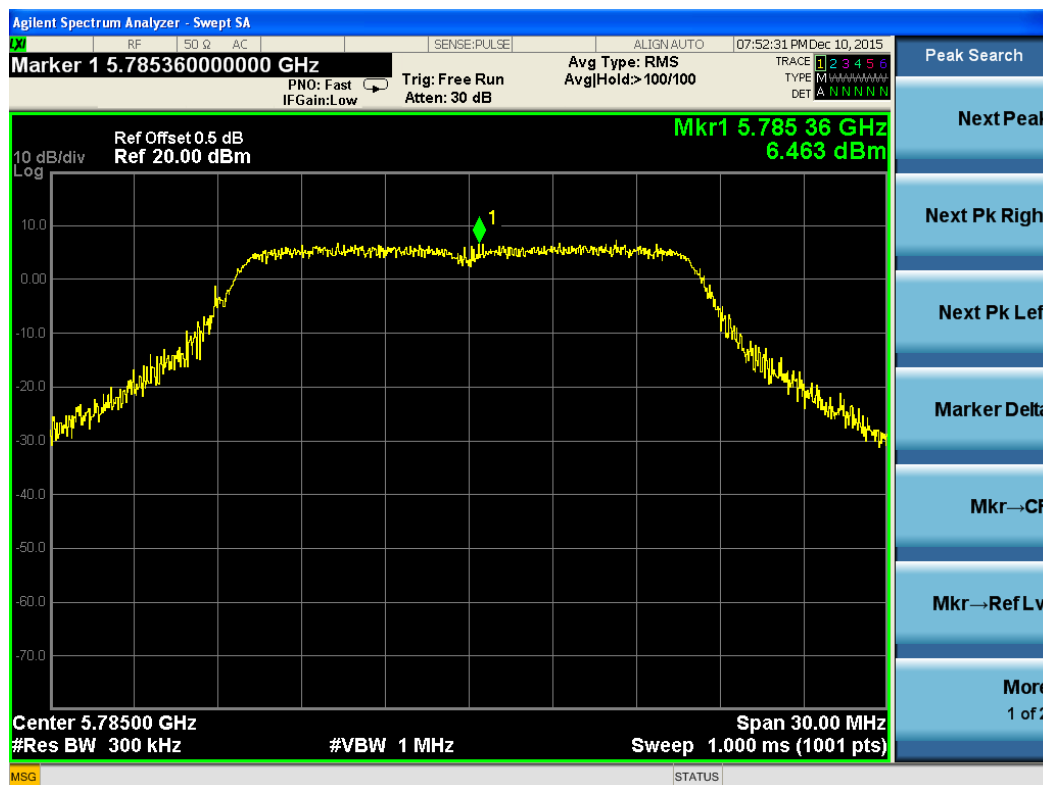
Test Plot For 802.11a-5785M-Chain 3
