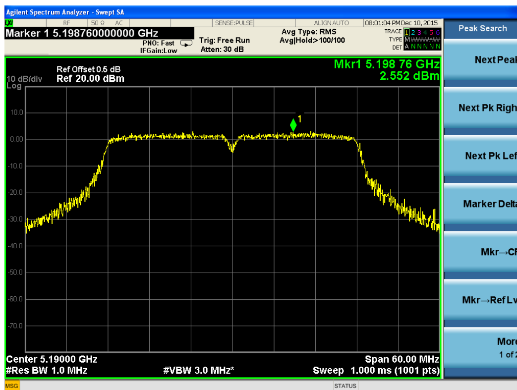
Test Plot For 802.11n(HT40)-5190M-Chain 1
