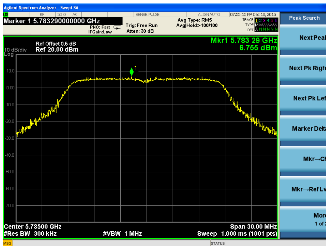
Test Plot For 802.11n(HT20)-5785M-Chain 1
