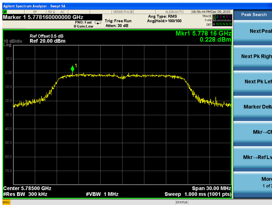
Test Plot For 802.11n(HT20)-5785M-Chain 2
