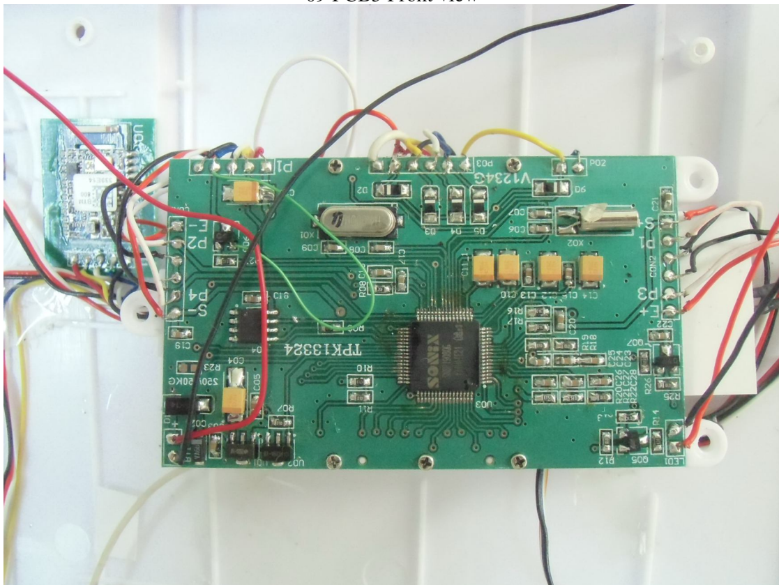
09 PCB3 Front view
