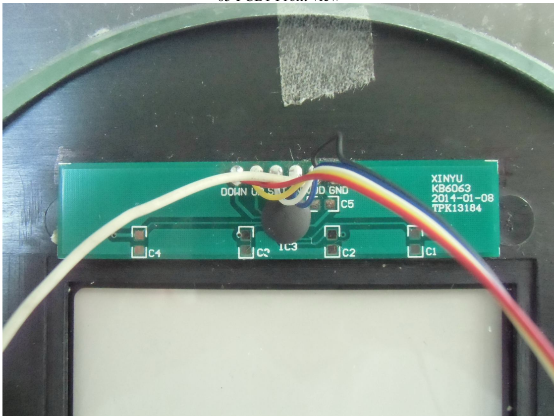
05 PCB1 Front view
