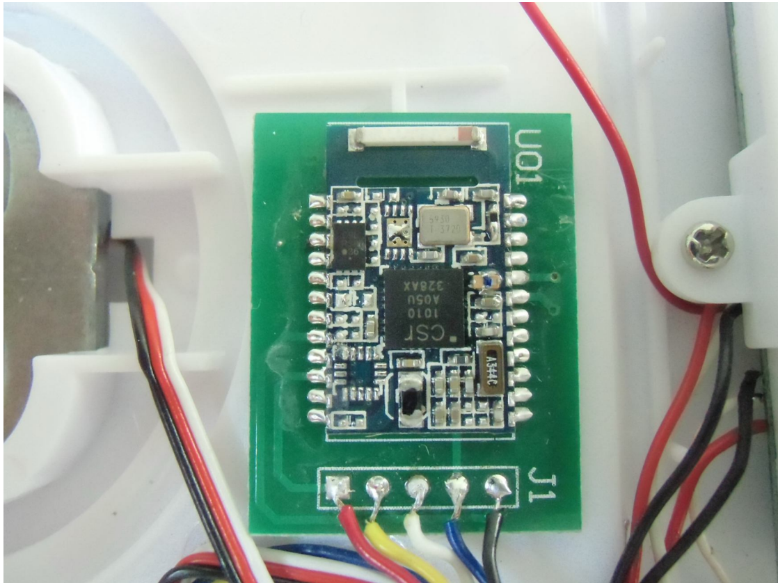
07 PCB2 Front view
