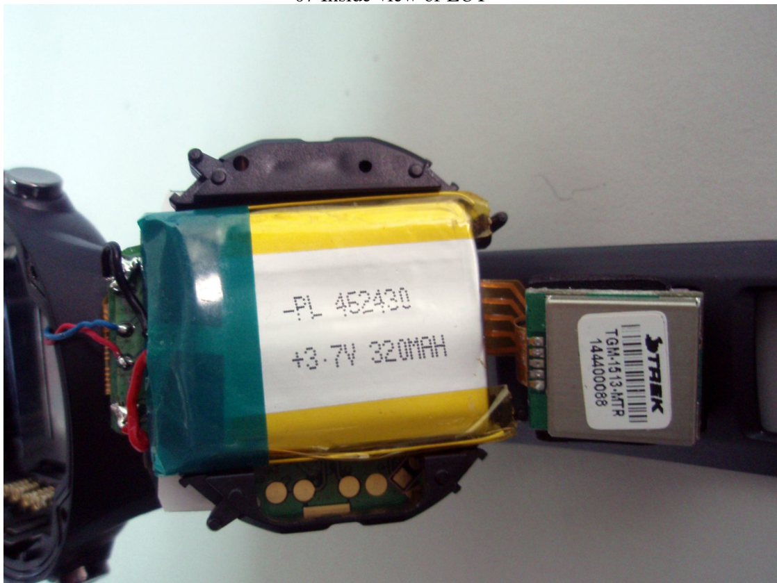
07 Inside view of EUT
