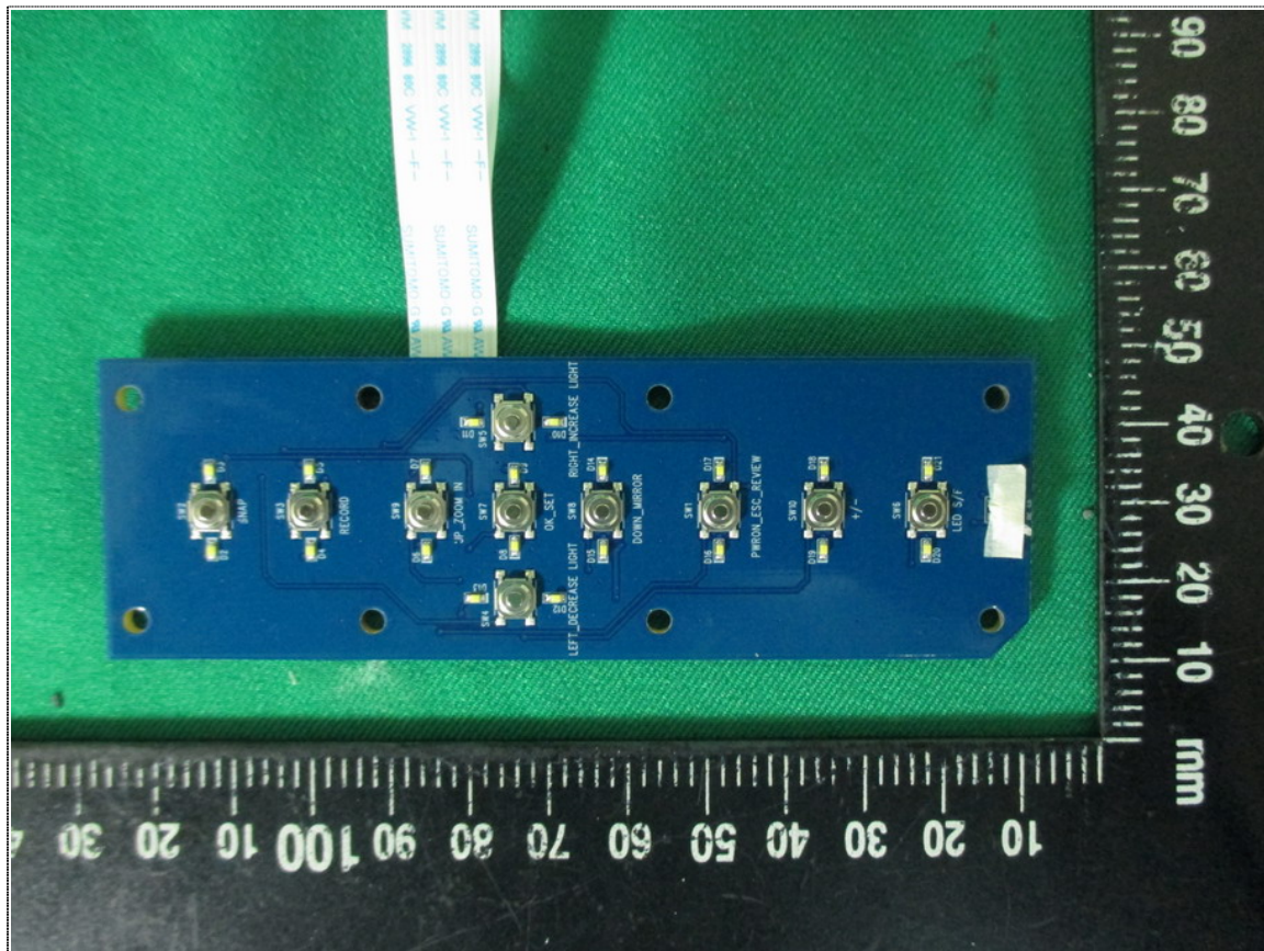
Component View of Button Board
