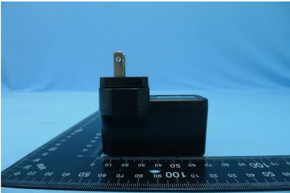
(18) Adapter Photo
