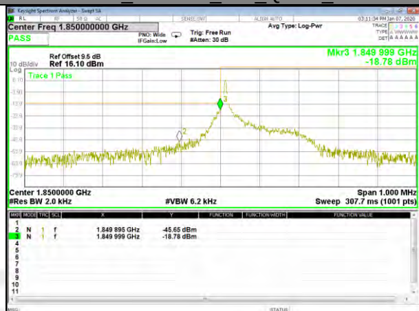
Band 2_3.75KHz_1#47_QPSK_High
