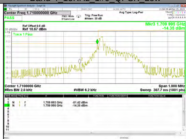
Band 4_15KHz_1#0_QPSK_Low
