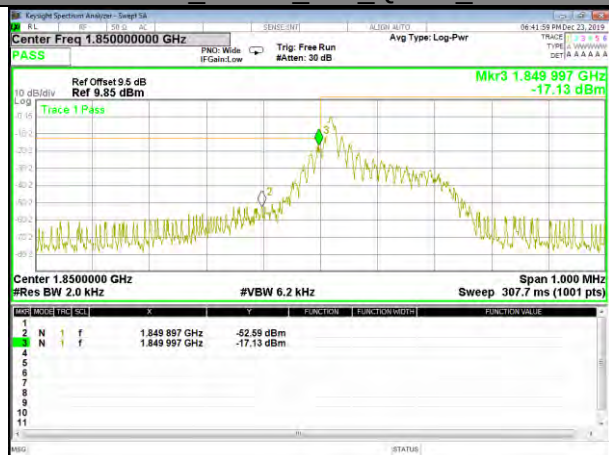
Band 2_15KHz_1#0_QPSK_Low
