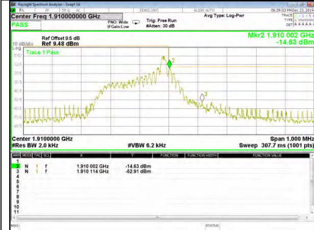
Band 2_15KHz_12#0_QPSK_High
