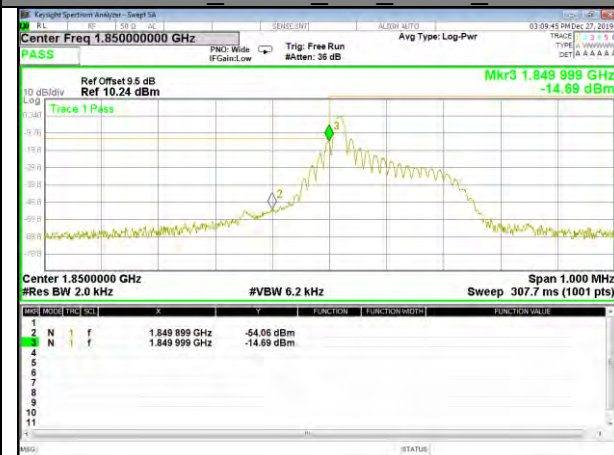
Band 25_15KHz_1#0_BPSK_Low
