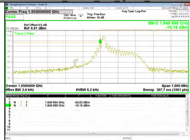
Band 25_15KHz_1#0_QPSK_Low
