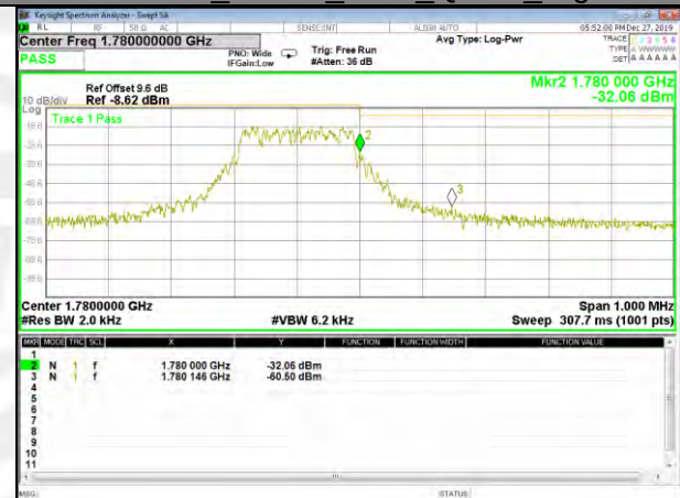
Band 66_15KHz_12#0_QPSK_High
