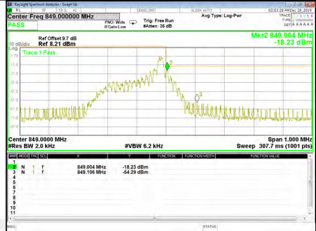
Band 5_15KHz_12#0_QPSK_High
