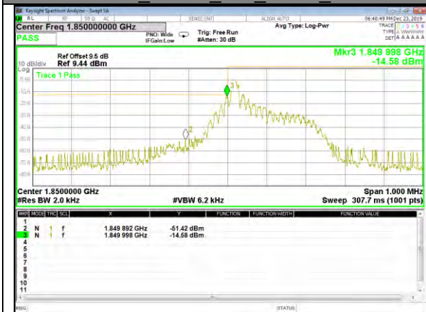
Band 2_15KHz_1#0_BPSK_Low
