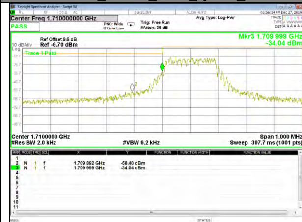
Band 66_15KHz_12#0_QPSK_Low
