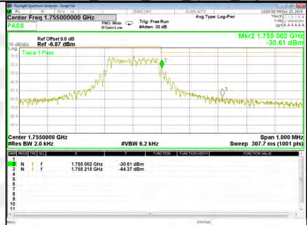
Band 4_15KHz_12#0_QPSK_High
