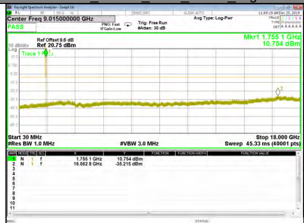
Band 4_15KHz_1#11_BPSK_High
