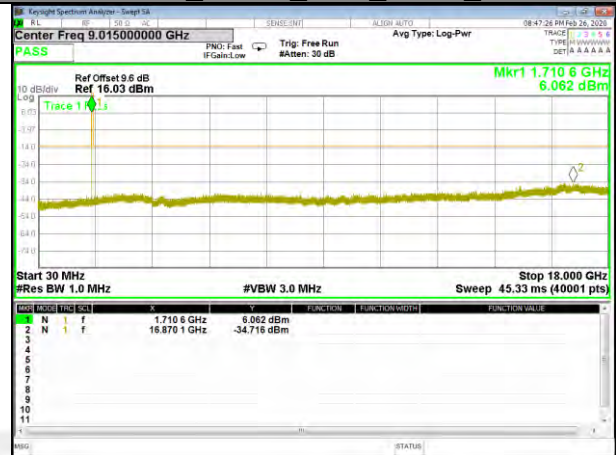
Band 4_15KHz_1#11_BPSK_Mid
