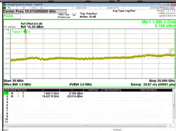
Band 2_3.75KHz_1#47_QPSK_Mid
