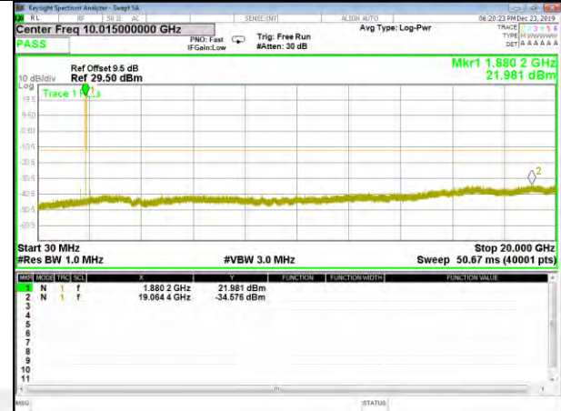
Band 2_15KHz_12#0_QPSK_Mid
