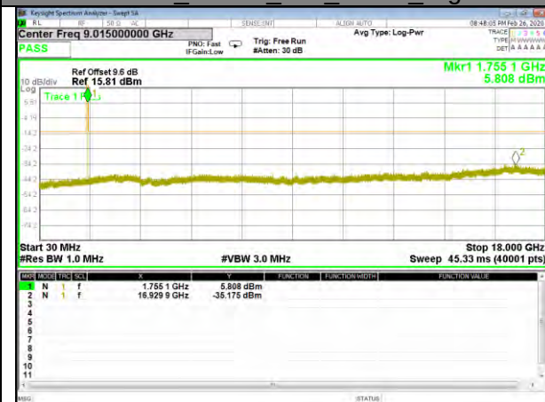
Band 4_15KHz_1#0_BPSK_High
