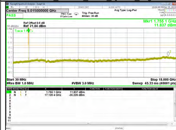
Band 4_15KHz_12#0_QPSK_High
