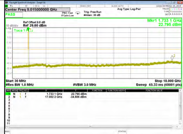
Band 4_15KHz_12#0_QPSK_Mid
