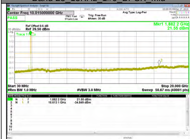
Band 25_15KHz_1#0_BPSK_Mid
