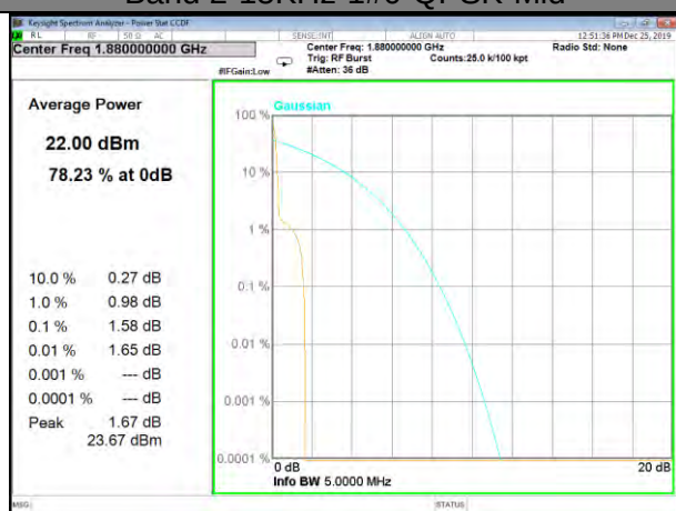
Band 2-15KHz-1#0-QPSK-Mid
