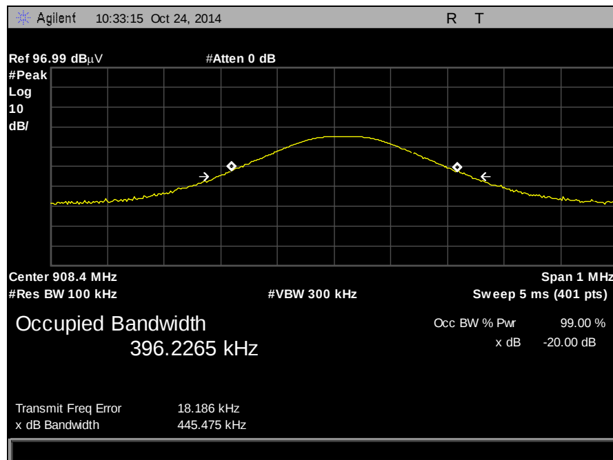
Plot 7. 20 dB Occupied Bandwidth
