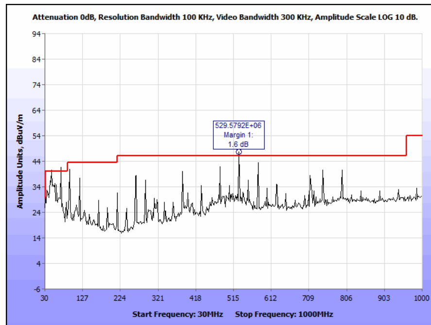
Plot 9. Radiated Spurious Emissions, Radio Off
