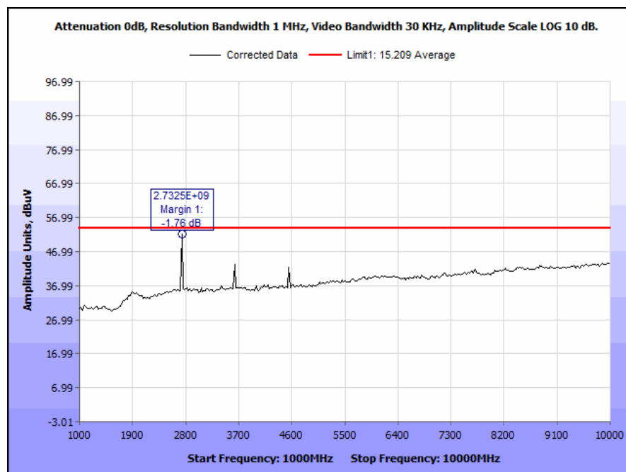
Plot 11. Radiated Spurious Emissions, 1 GHz – 10 GHz, Average
