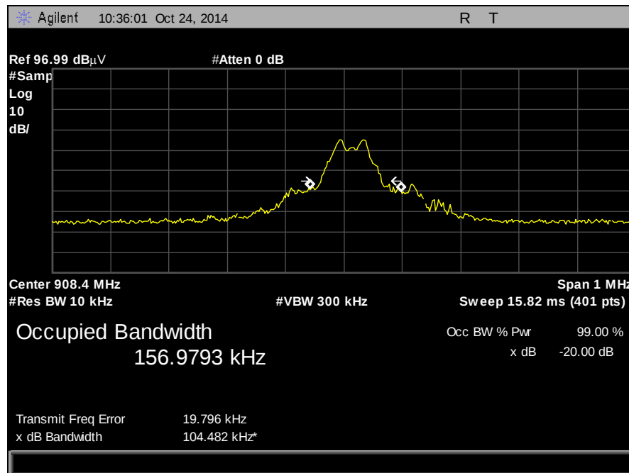
Plot 8. 99 % dB Occupied Bandwidth
