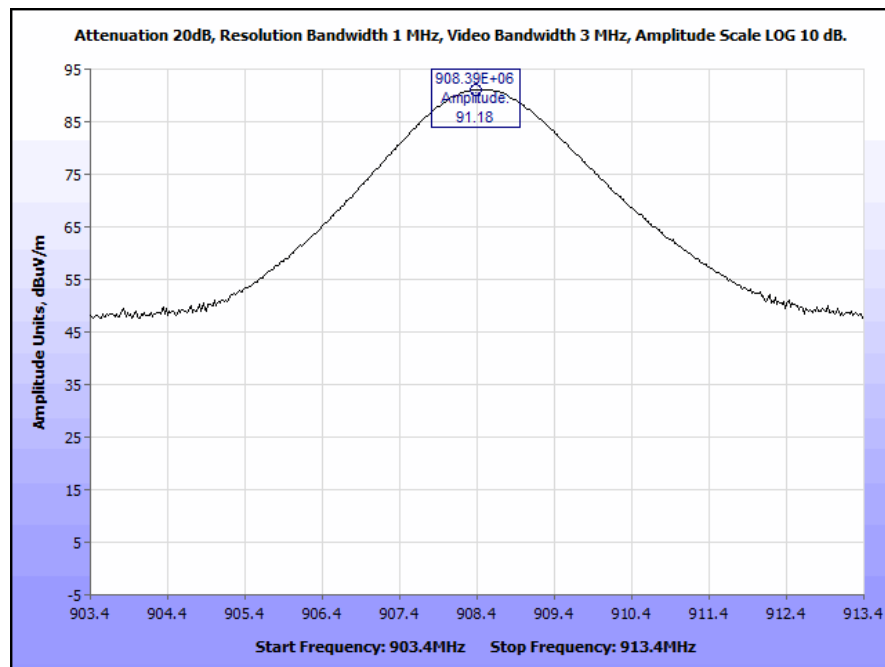
Plot 6. Radiated Field Strength of Fundamental
