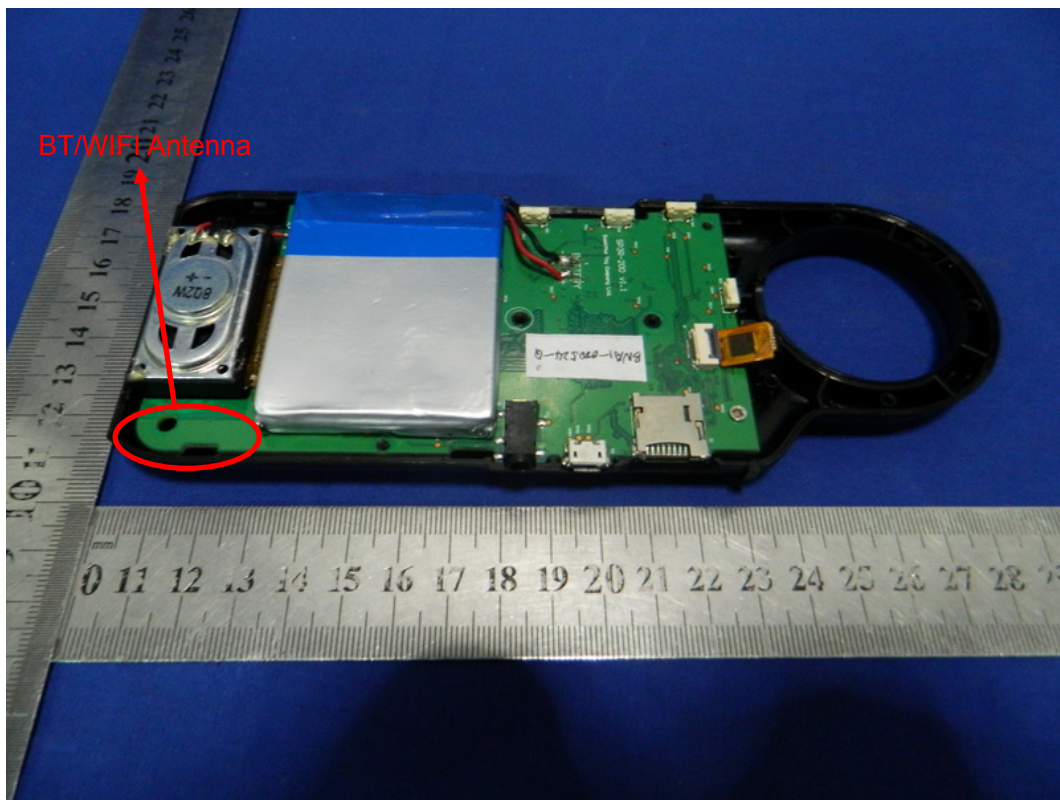
b: Antenna Schemes(Back Side of EUT)
