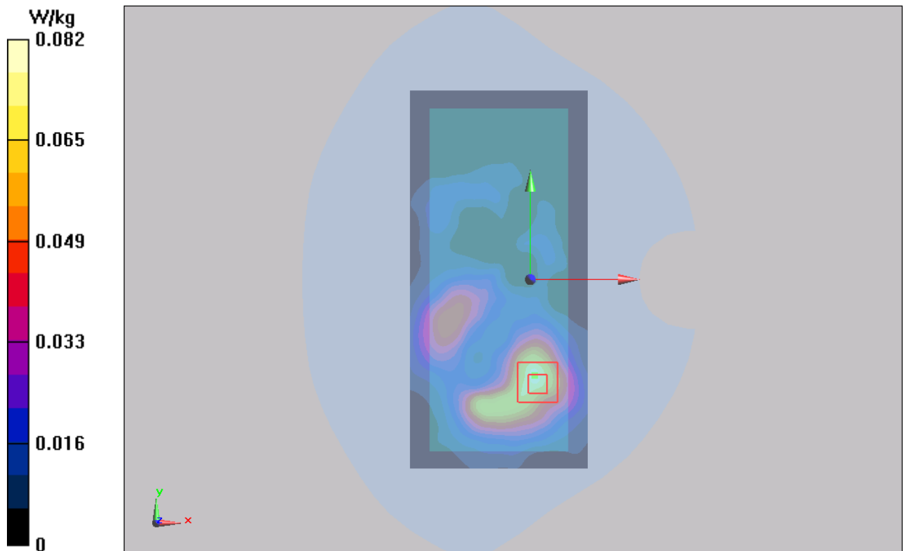
Figure 7 802.11b Test Position 1 Channel 6
