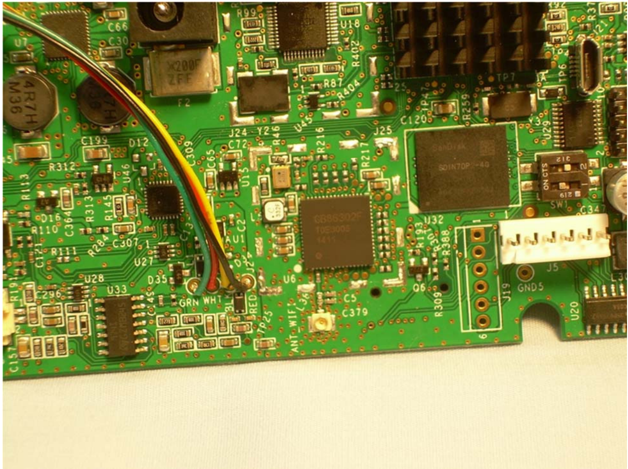
View of Back Side of Main PCB Circuitry with RF Shield Removed
