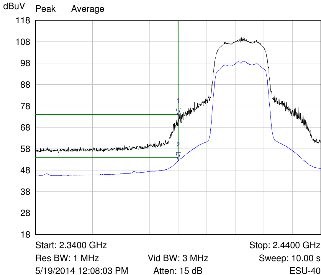
Channel 1 Band Edge Plot (802.11n)
