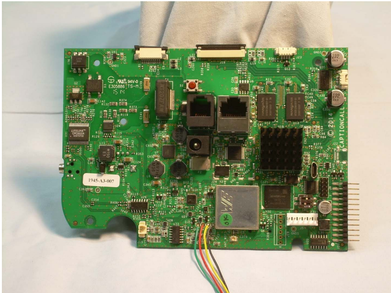
Photograph 10 – View of the Back Side of the Main PCB
