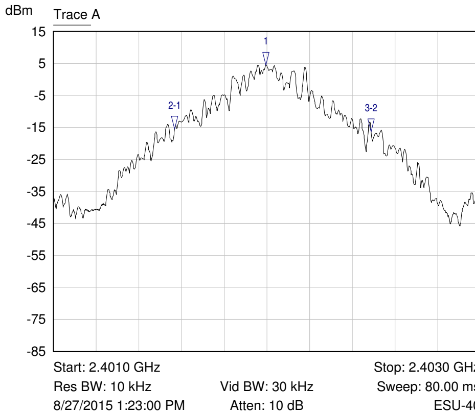
Lowest Channel 20 dB Bandwidth – SDR
