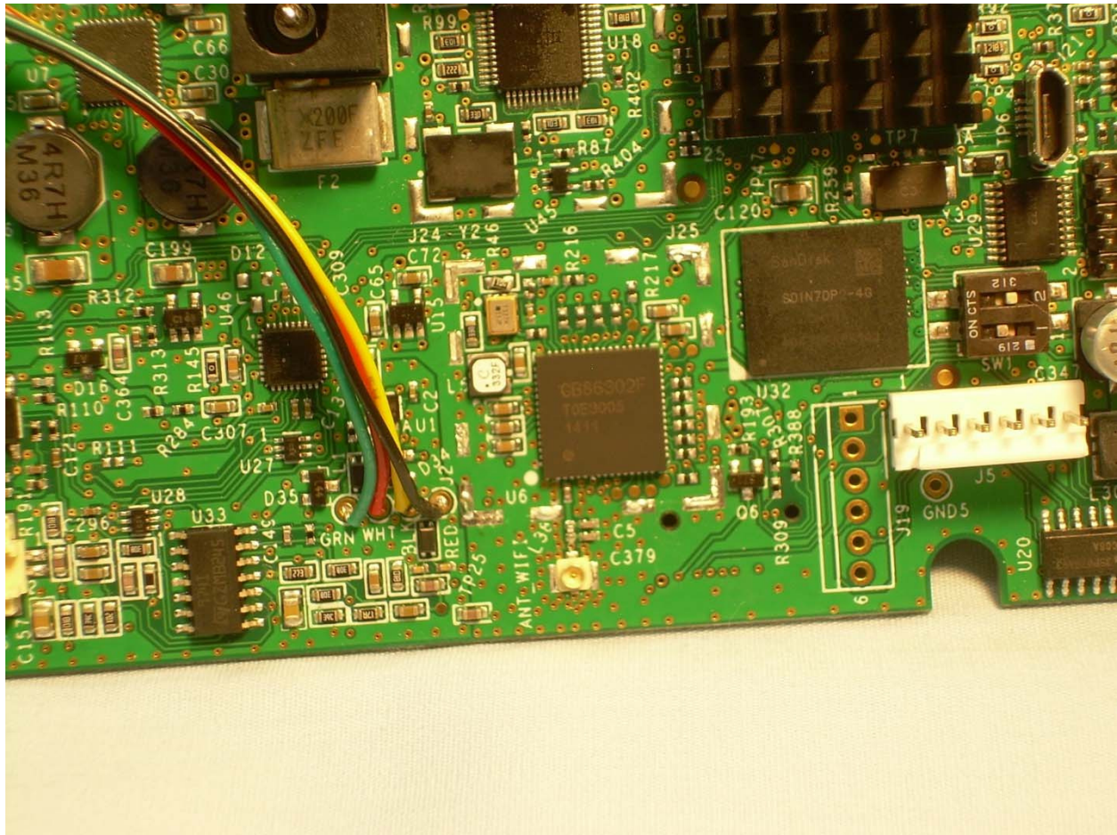
Photograph 11 – View of the Back Side of the Main PCB Circuitry with RF Shield Removed
