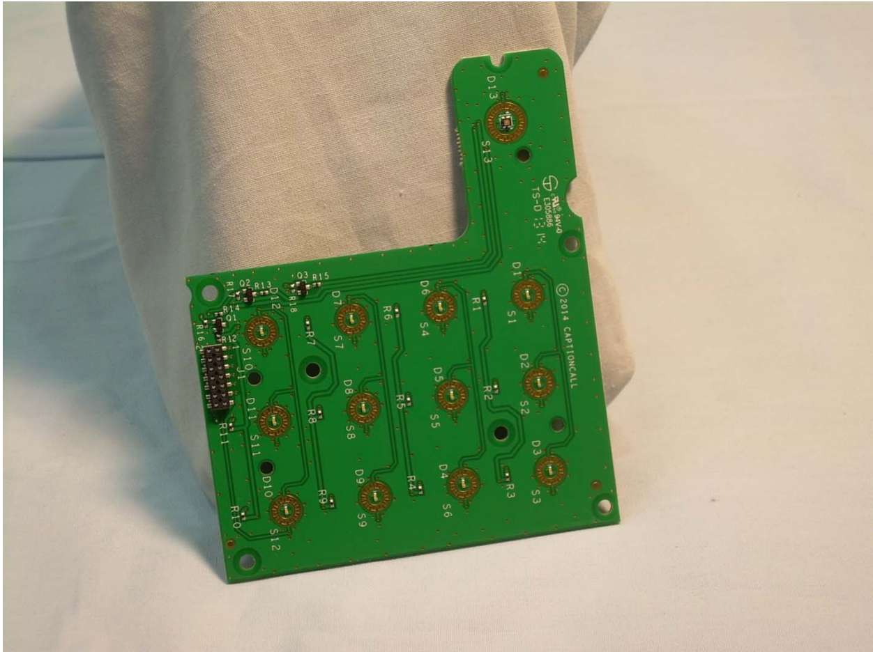
Photograph 16 – View of the Front Side of the Button Interface PCB
