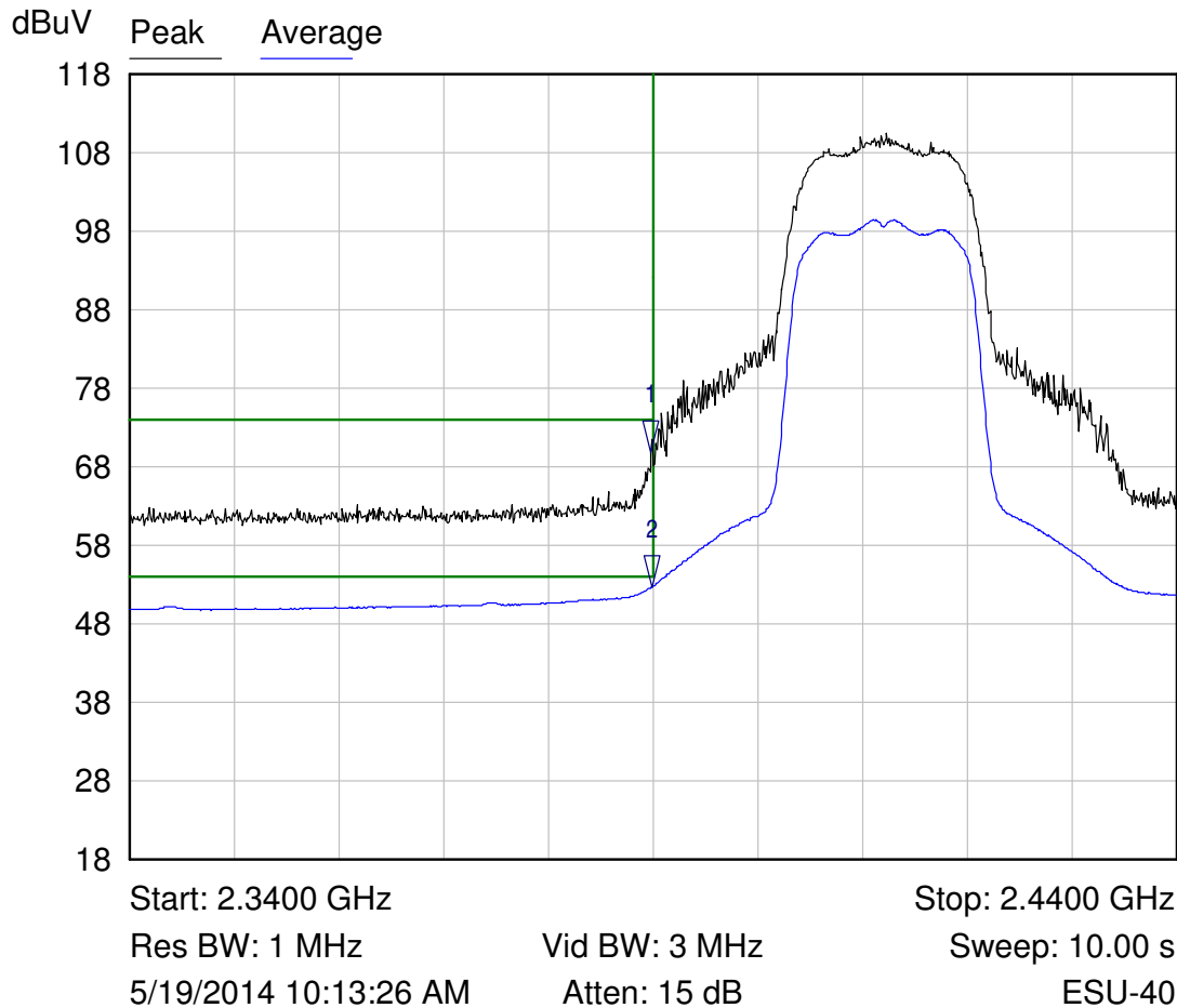
Channel 1 Band Edge Plot (802.11g)
