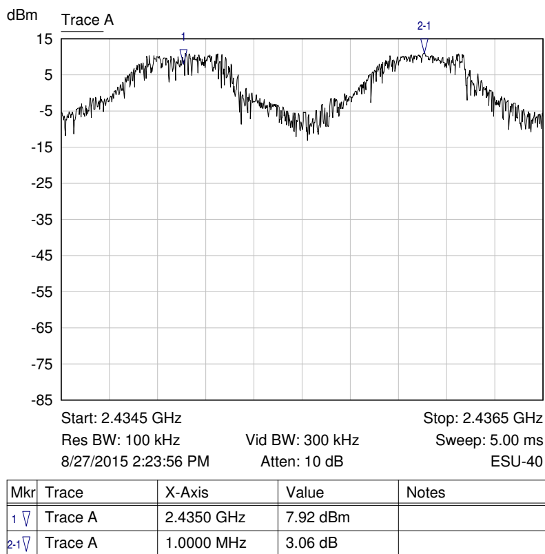
Channel Separation Plot
