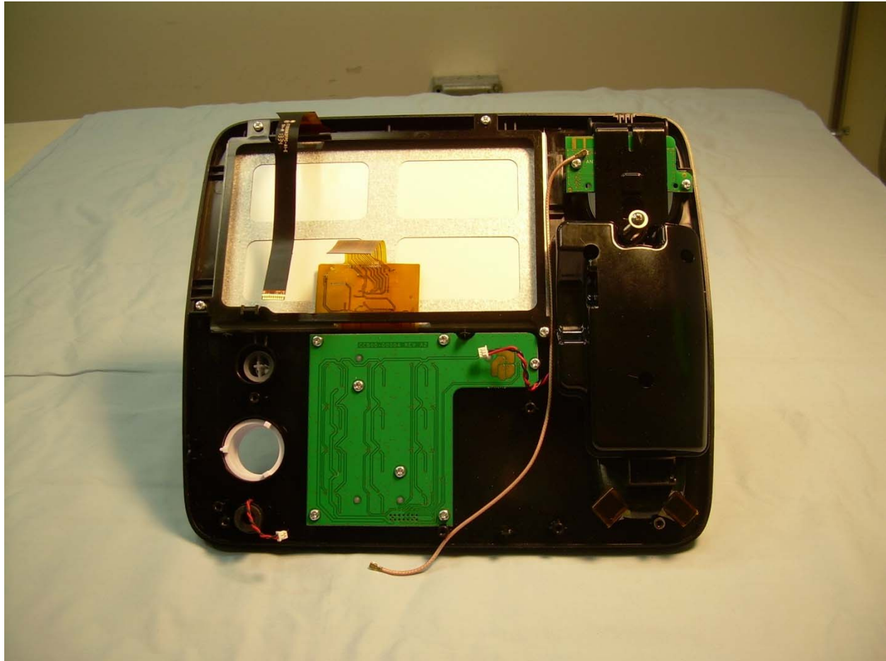
Photograph 18 – Internal View of the EUT with the Main PCB Removed
