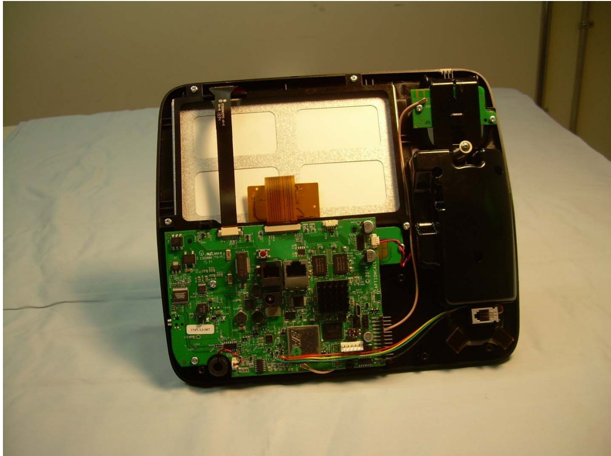
Photograph 9 – View of the EUT with the Back Cover Removed
