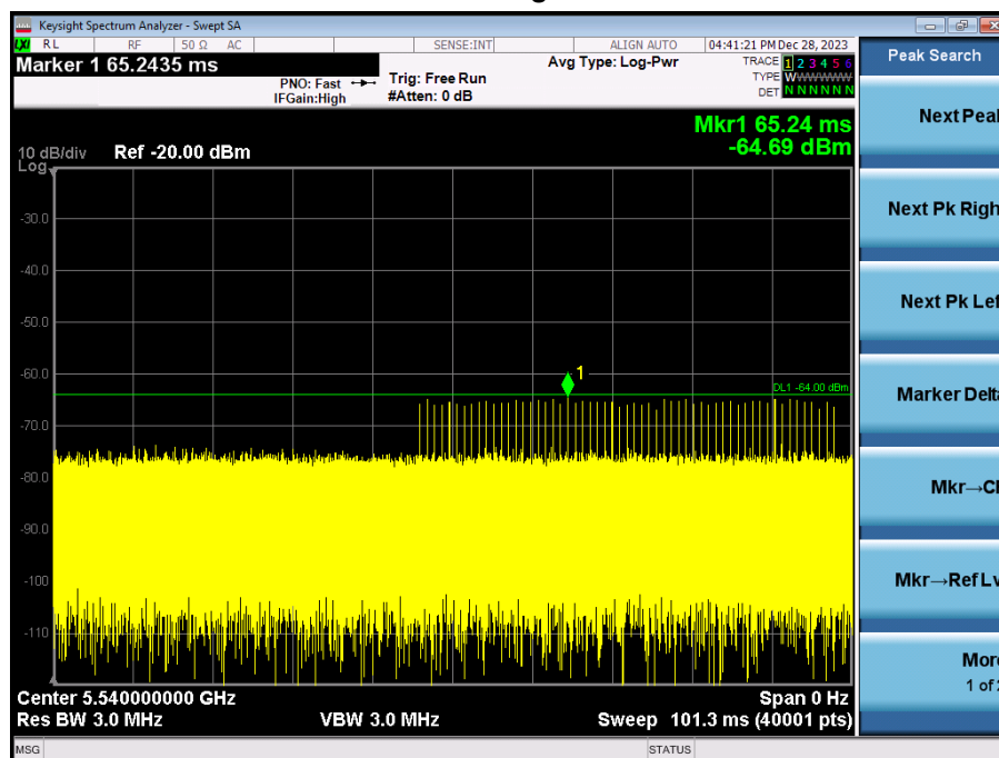
Radar Signal 1
