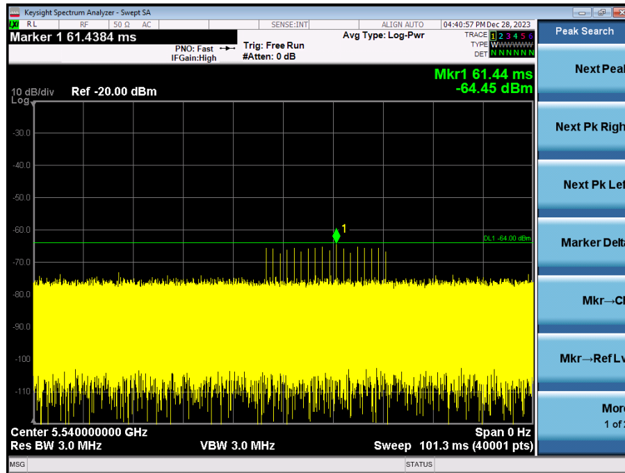
Radar Signal 0
