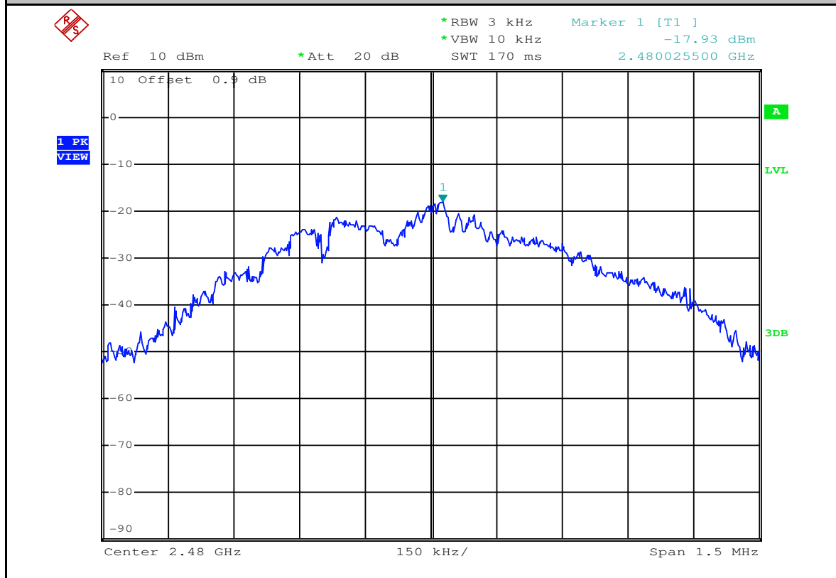
Maximum Peak power spectral density_BLE_2480_Ant1
