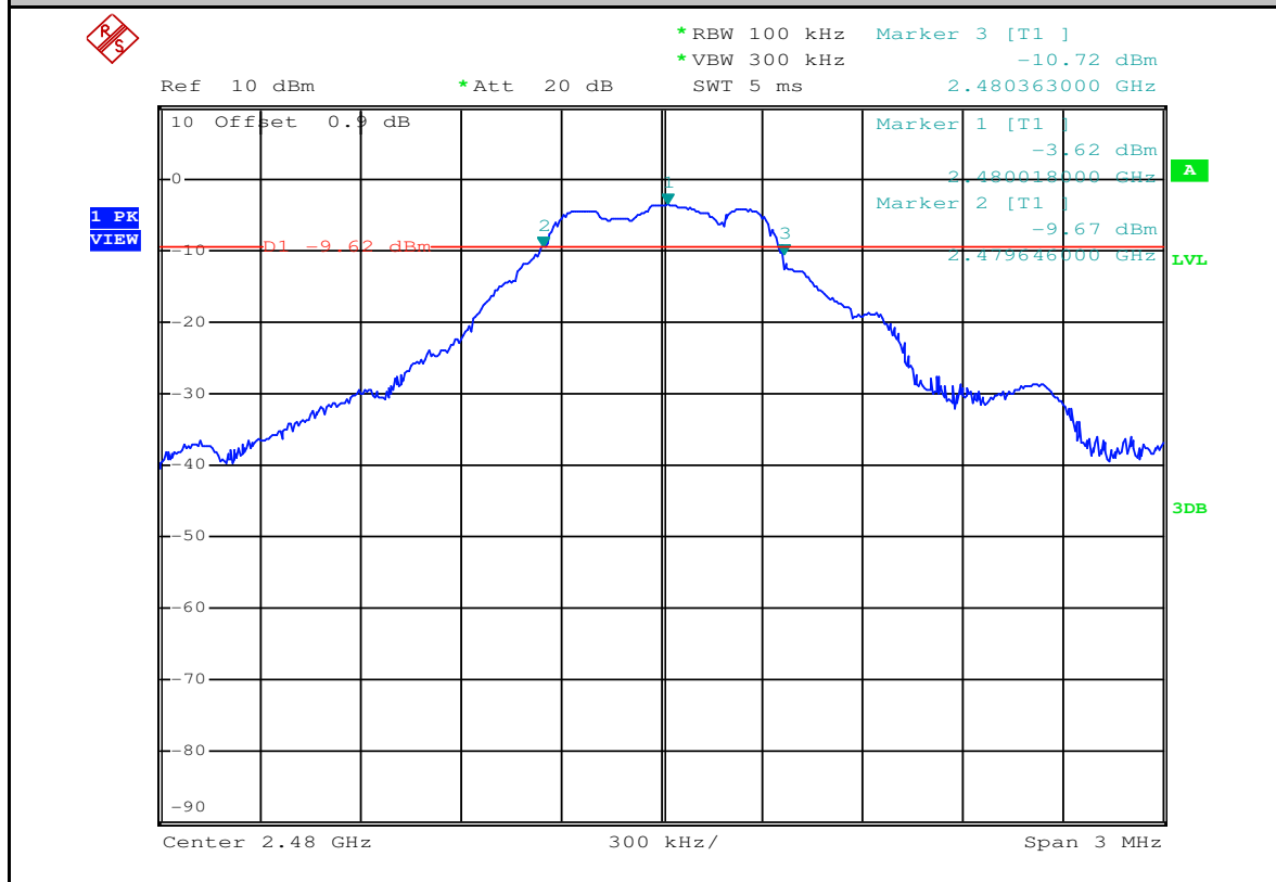
6dB Bandwidth_BLE_2480_Ant1
