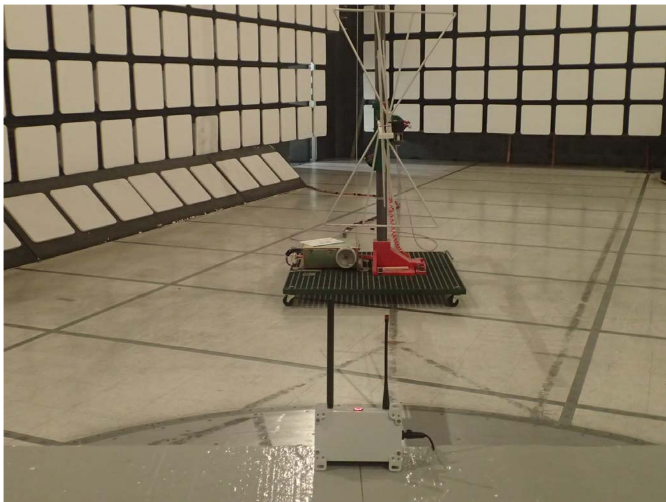
Radiated Emissions at 3m Distance EUT Orientation: Orthogonal Position 2
