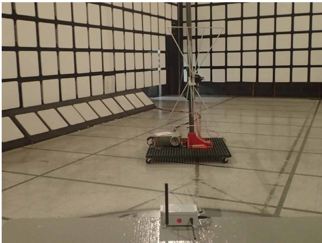
Radiated Emissions at 3m Distance EUT Orientation: Orthogonal Position 1
