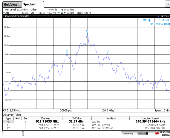
Figure 7.2.2-3: 911.75 MHz – IS0B
