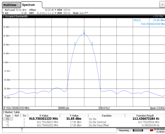
Figure 7.2.2-6: 910.75 MHz – IS0-10374
