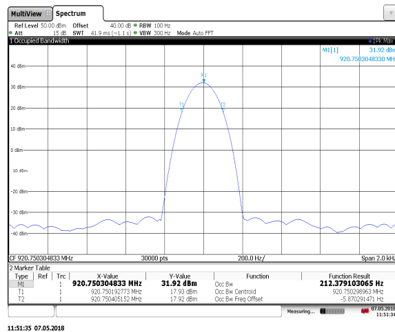
Figure 7.2.2-7: 920.75 MHz – IS0-10374
