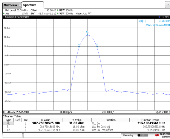
Figure 7.2.2-5: 902.75 MHz – IS0-10374
