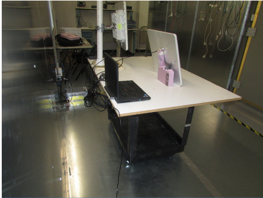
Figure 7: Conducted Emissions – Side - POE
