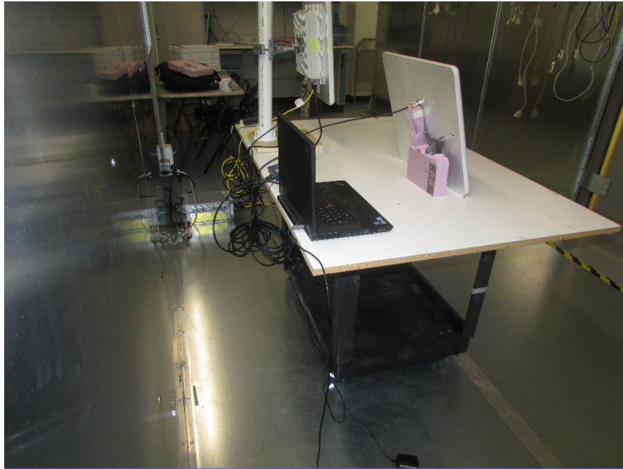
Figure 5: Conducted Emissions – Side - Power supply
