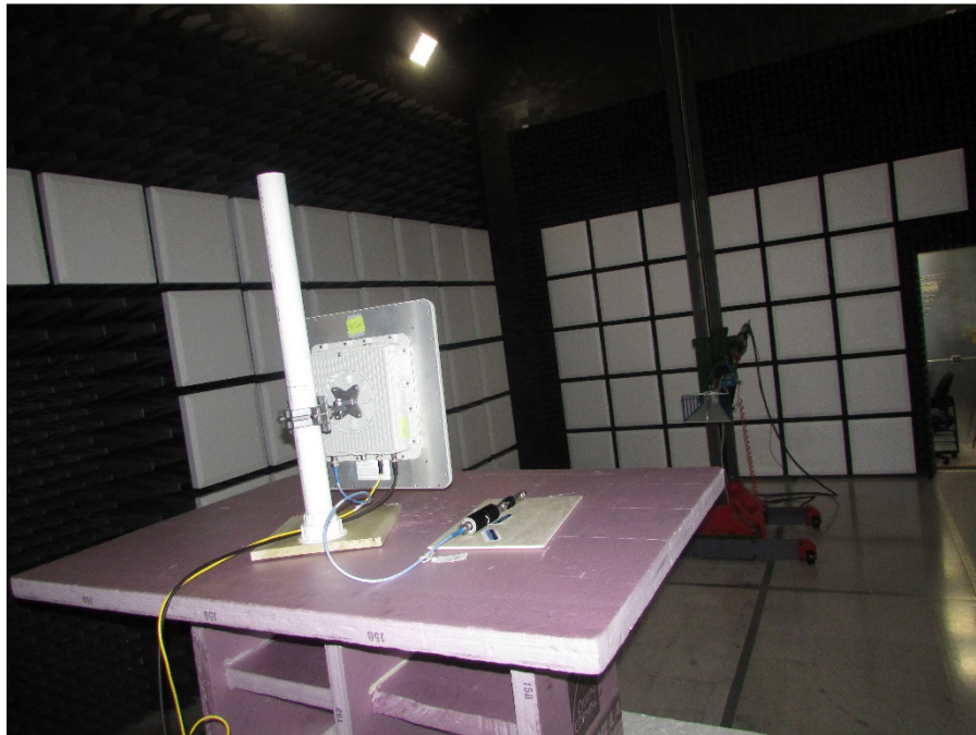
Figure 3: Radiated Emissions – Back – Above 1GHz
