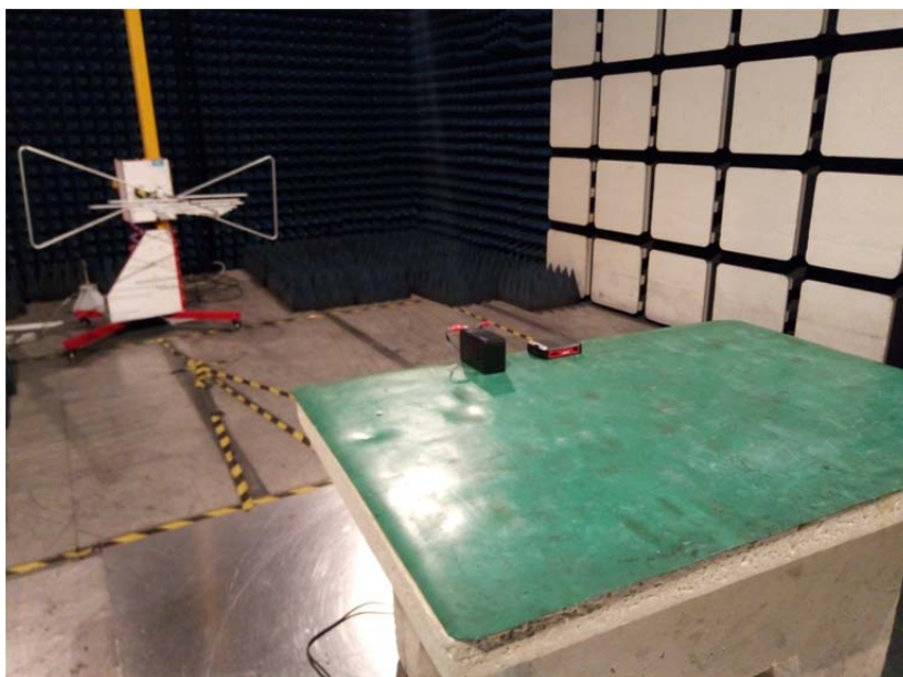
Test setup
