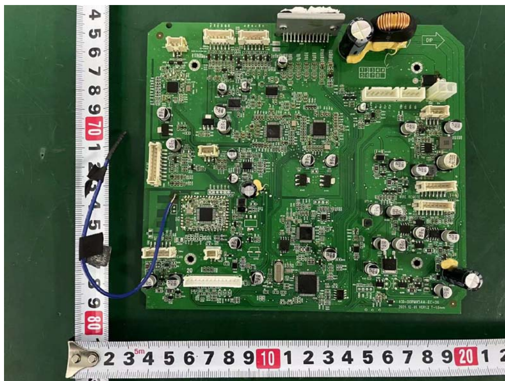
Internal photos M/N: PMX-5CAN
