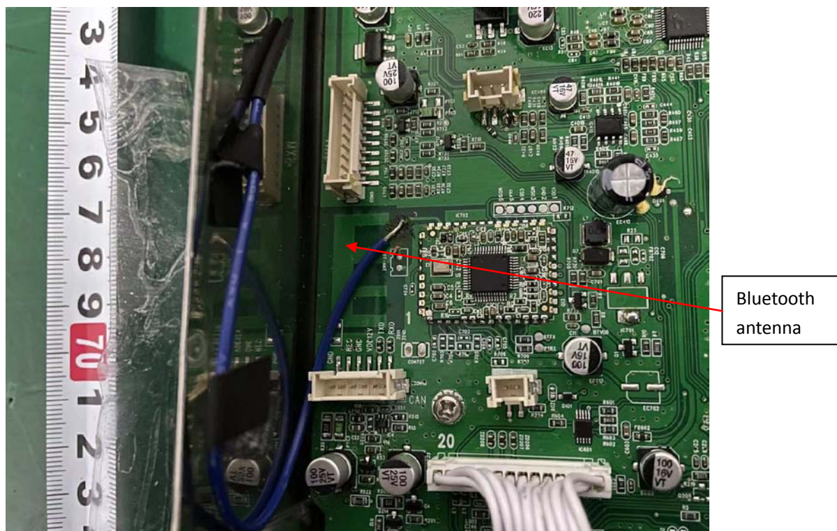
Internal photos M/N: PMX-5CAN
