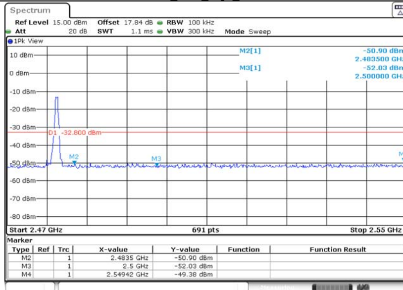
DH5_Ant1_High_2480
