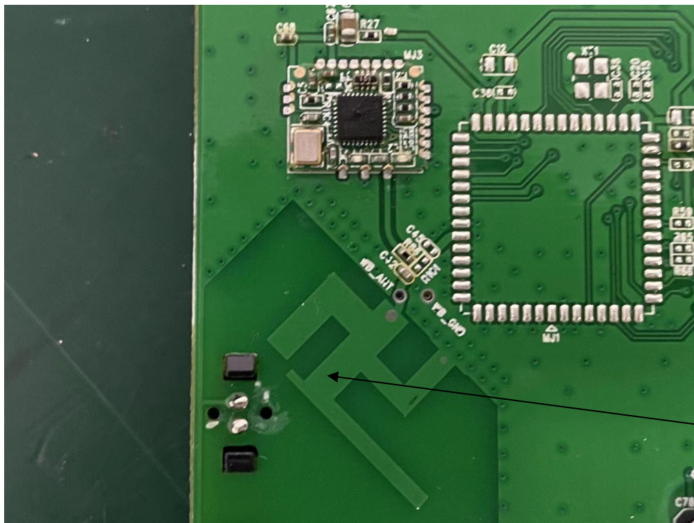
CW889 Bluetooth antenna
