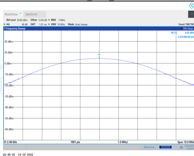
3DH5_Ant1_2480
