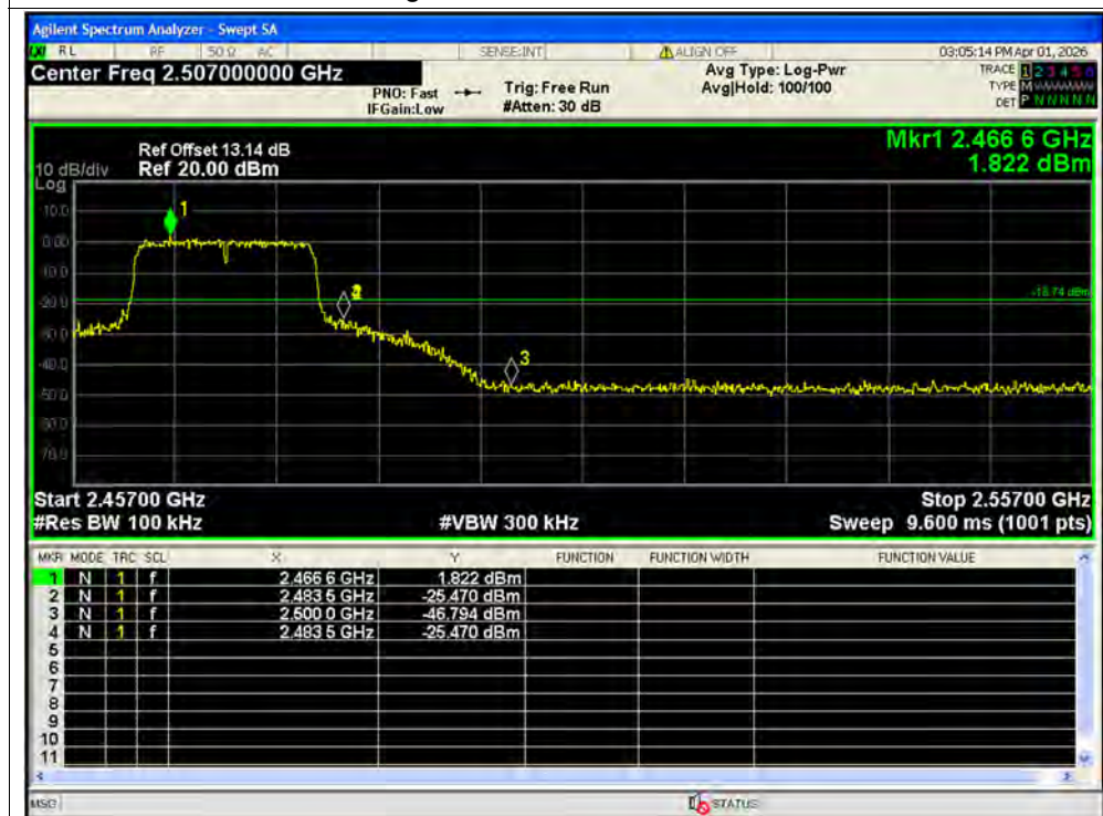
Band Edge NVNT n20 2472MHz Ant1 Emission
